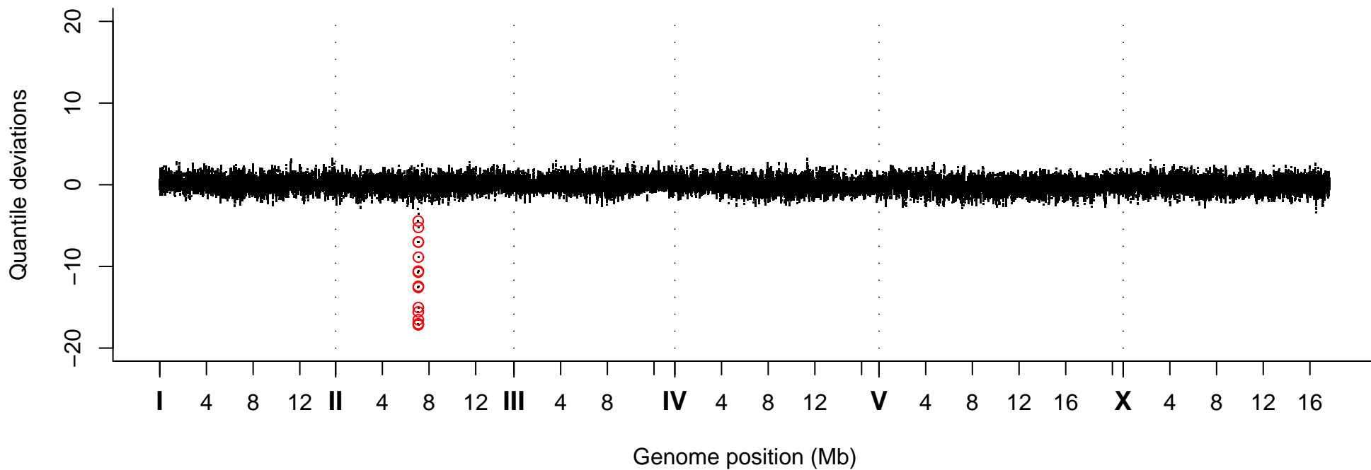
Quantile Deviations, Strain VC40451
