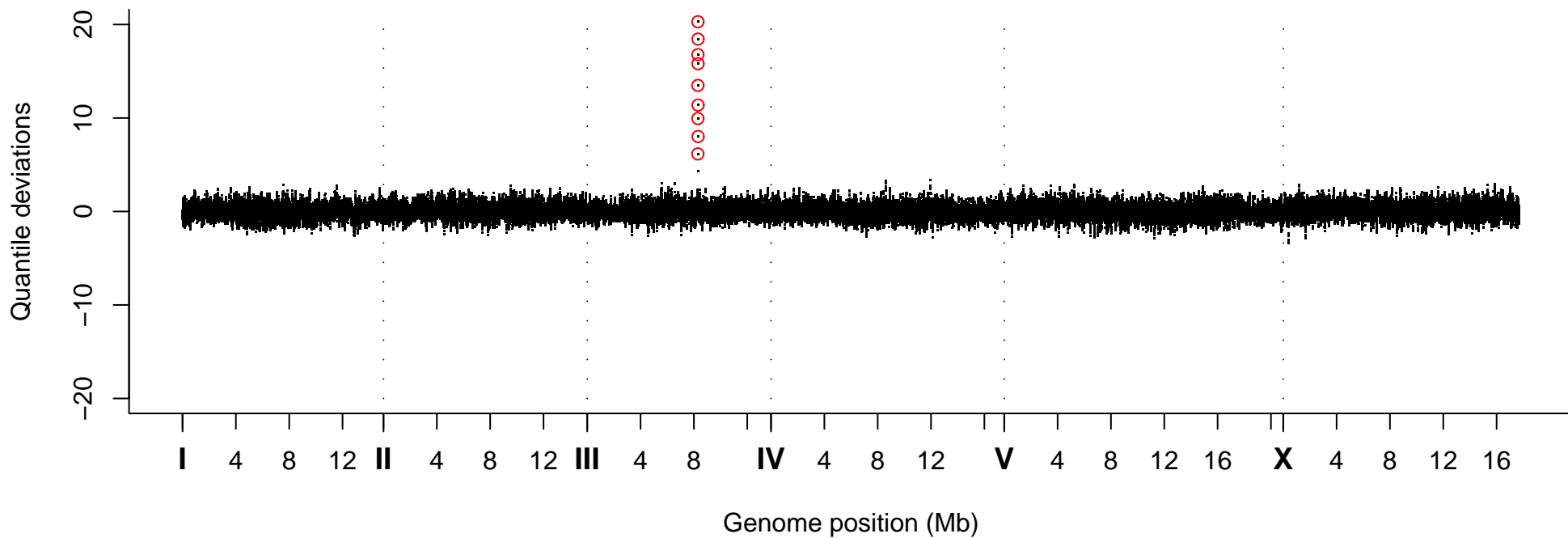
Quantile Deviations, Strain VC40453
