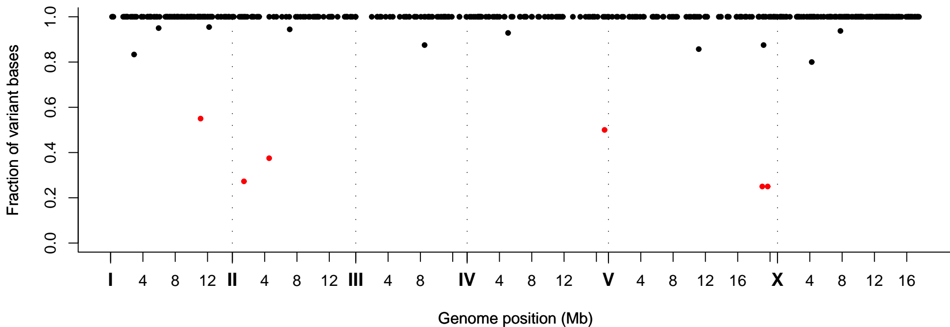
Fraction of Variant Bases at Position, Strain VC40453
