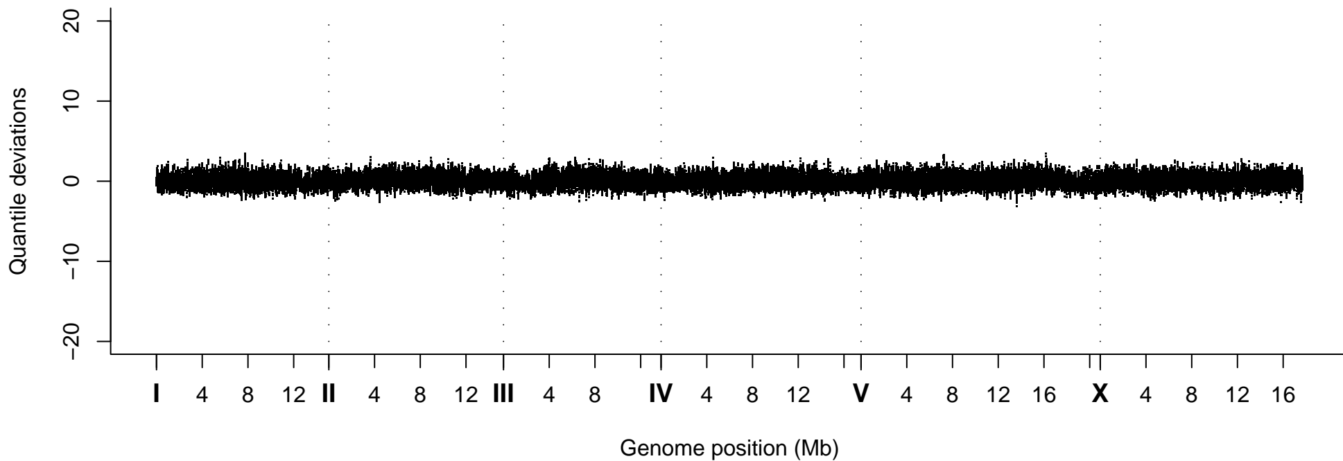
Quantile Deviations, Strain VC40454
