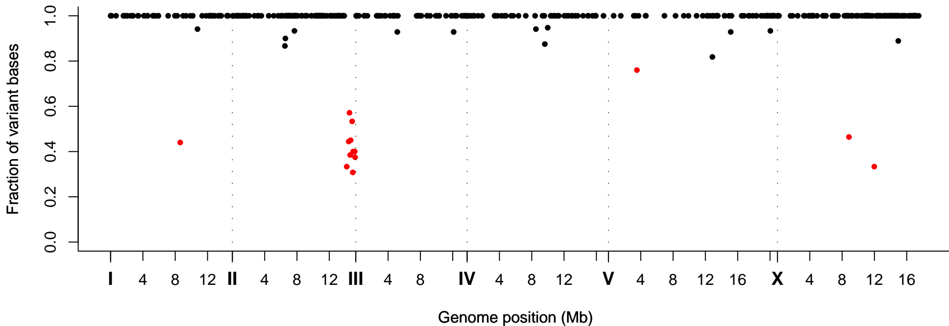
Fraction of Variant Bases at Position, Strain VC40454
