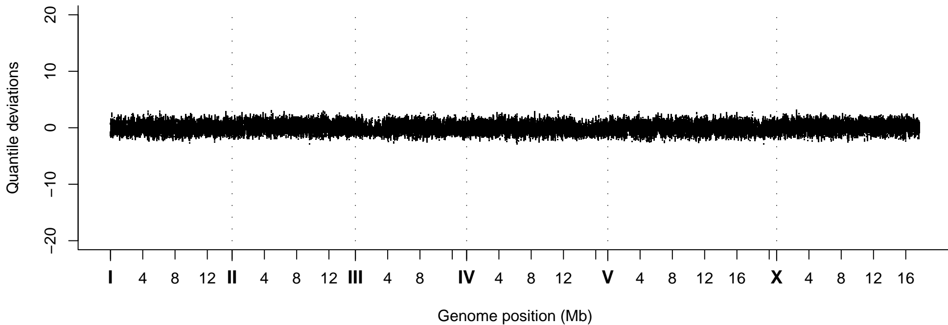
Quantile Deviations, Strain VC40459
