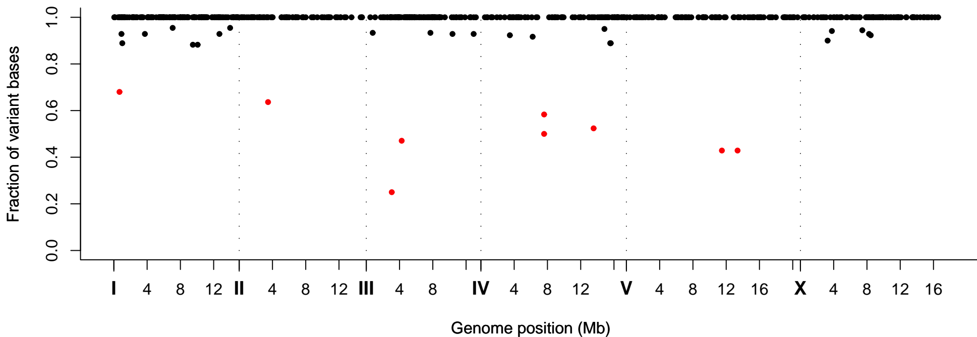
Fraction of Variant Bases at Position, Strain VC40459
