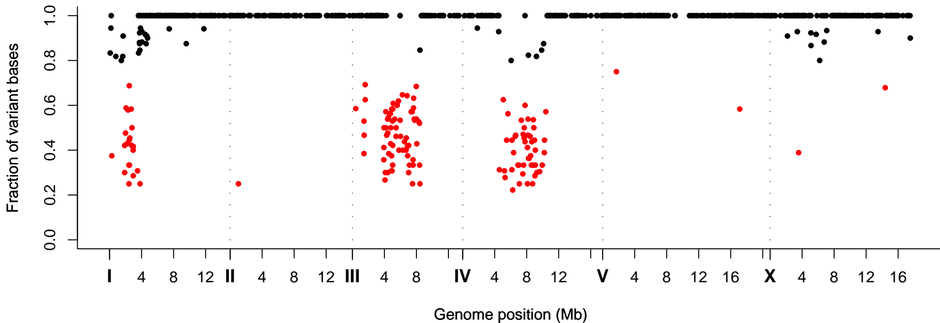
Fraction of Variant Bases at Position, Strain VC40467
