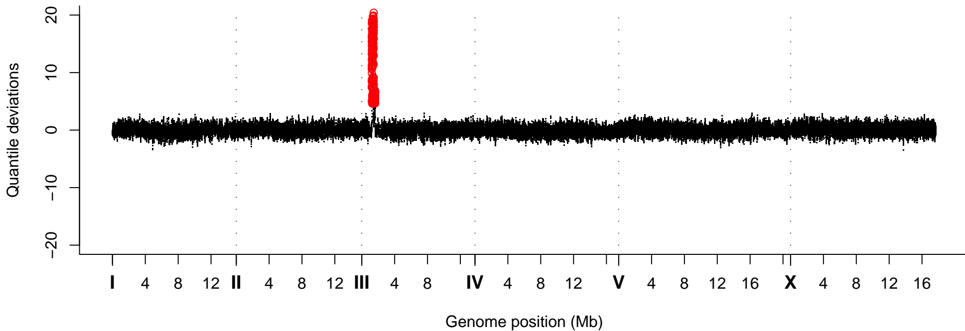
Quantile Deviations, Strain VC40467
