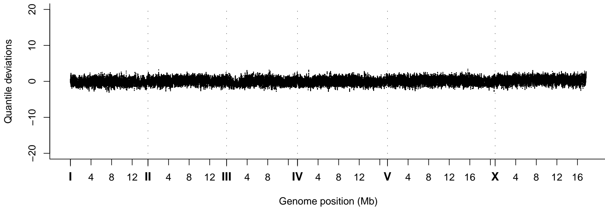
Quantile Deviations, Strain VC40474
