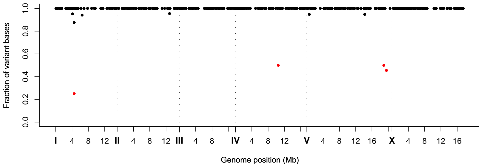
Fraction of Variant Bases at Position, Strain VC40474
