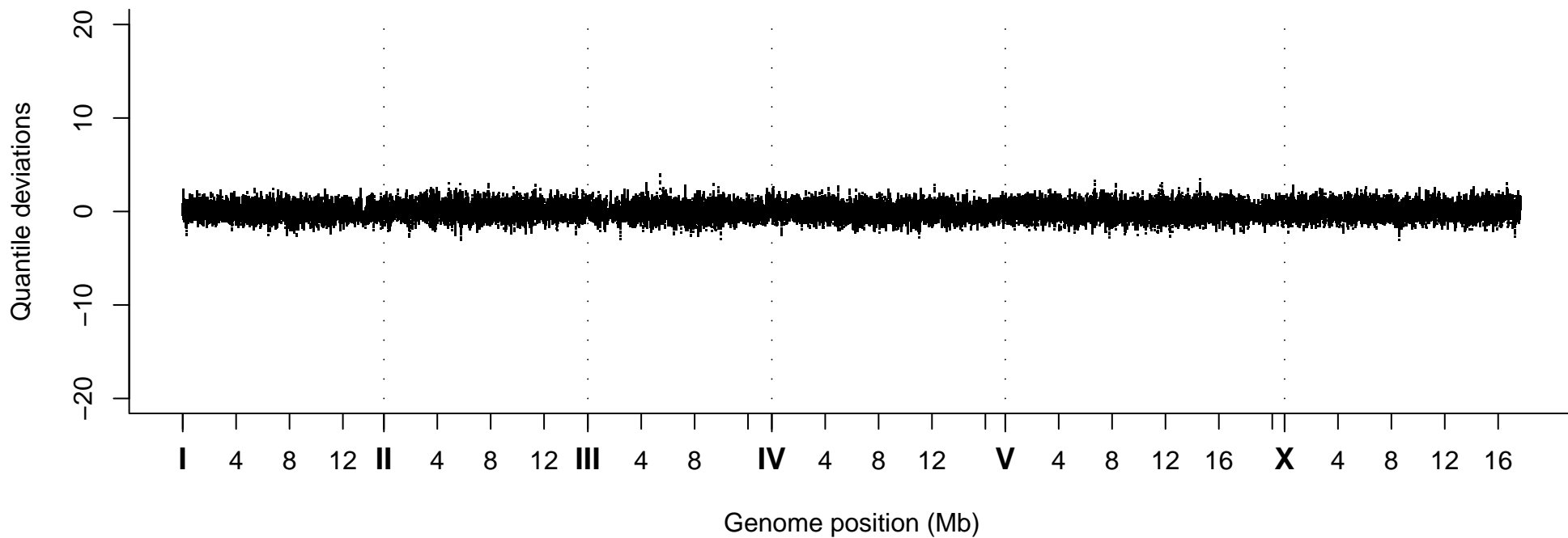
Quantile Deviations, Strain VC40475
