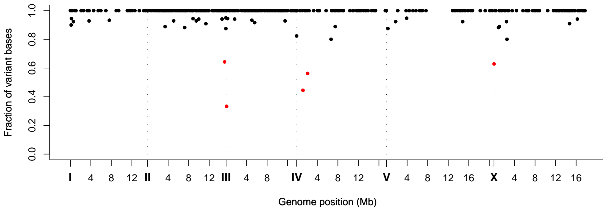
Fraction of Variant Bases at Position, Strain VC40475
