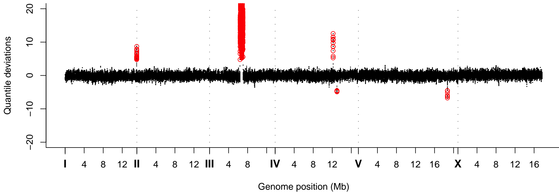
Quantile Deviations, Strain VC40485
