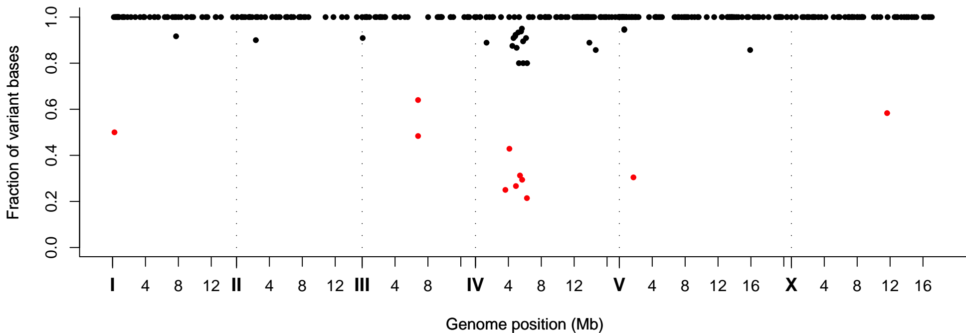
Fraction of Variant Bases at Position, Strain VC40485
