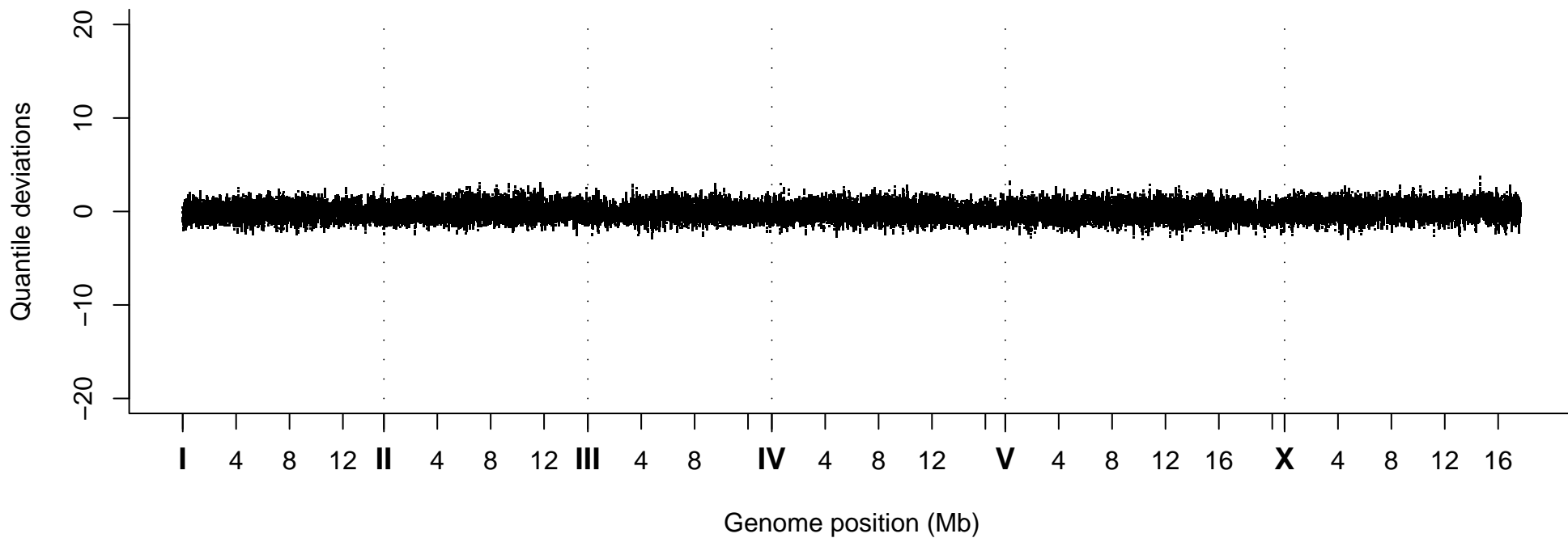
Quantile Deviations, Strain VC40488
