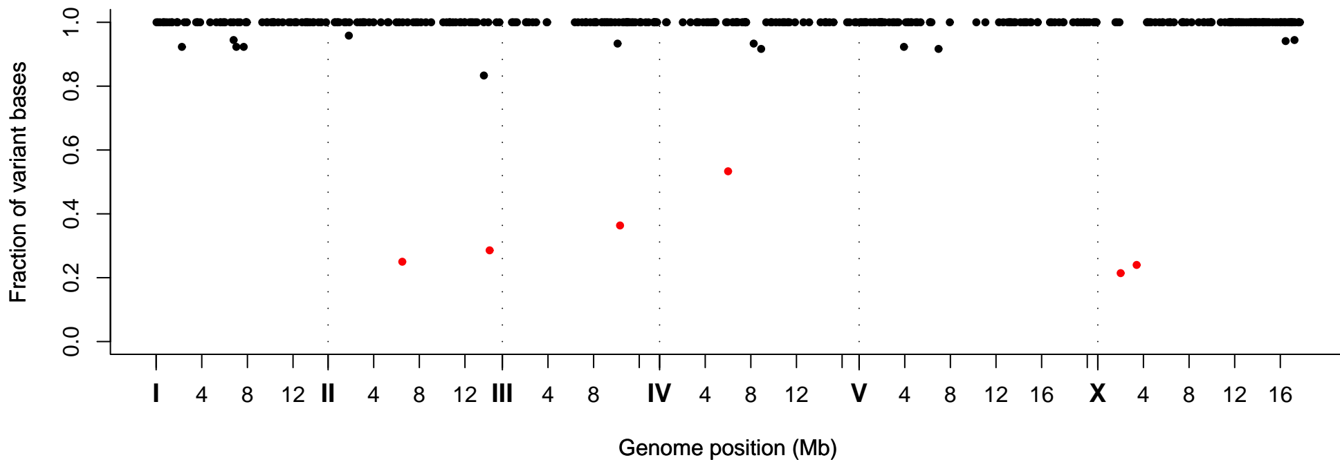
Fraction of Variant Bases at Position, Strain VC40488
