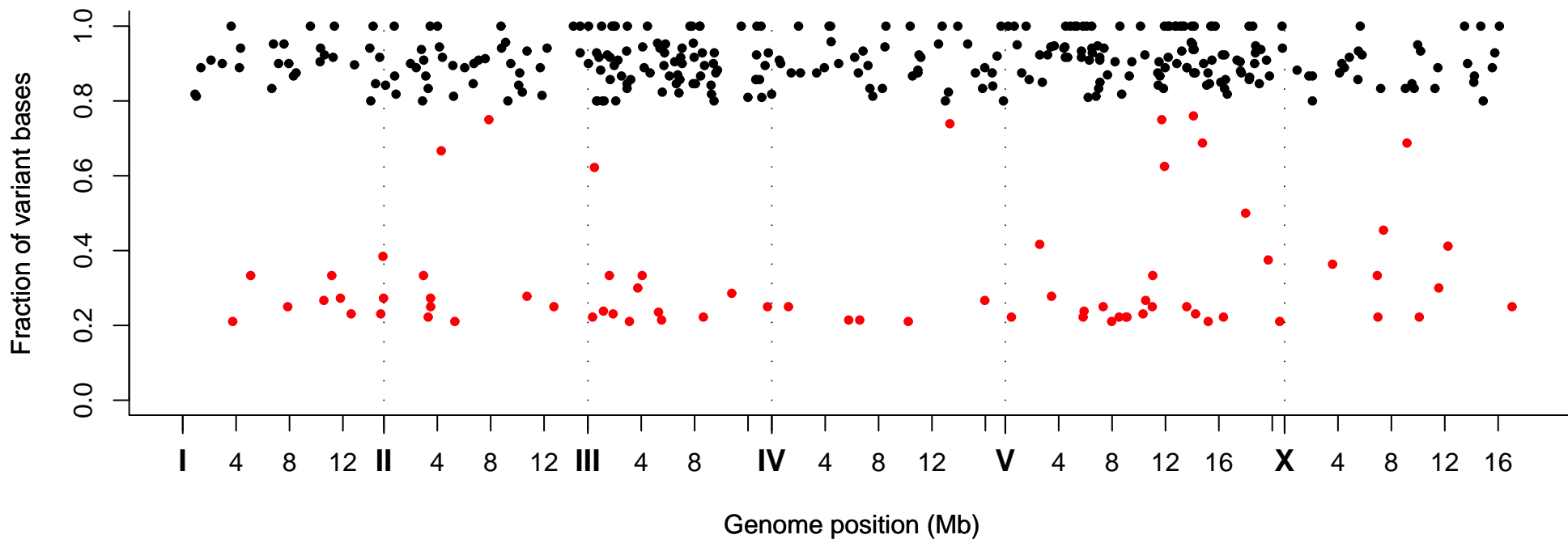
Fraction of Variant Bases at Position, Strain VC40491
