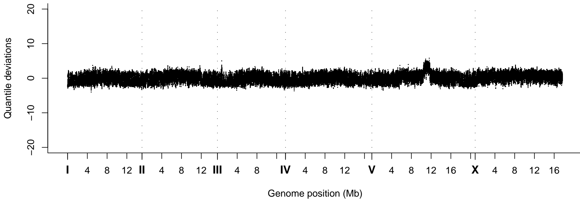
Quantile Deviations, Strain VC40491
