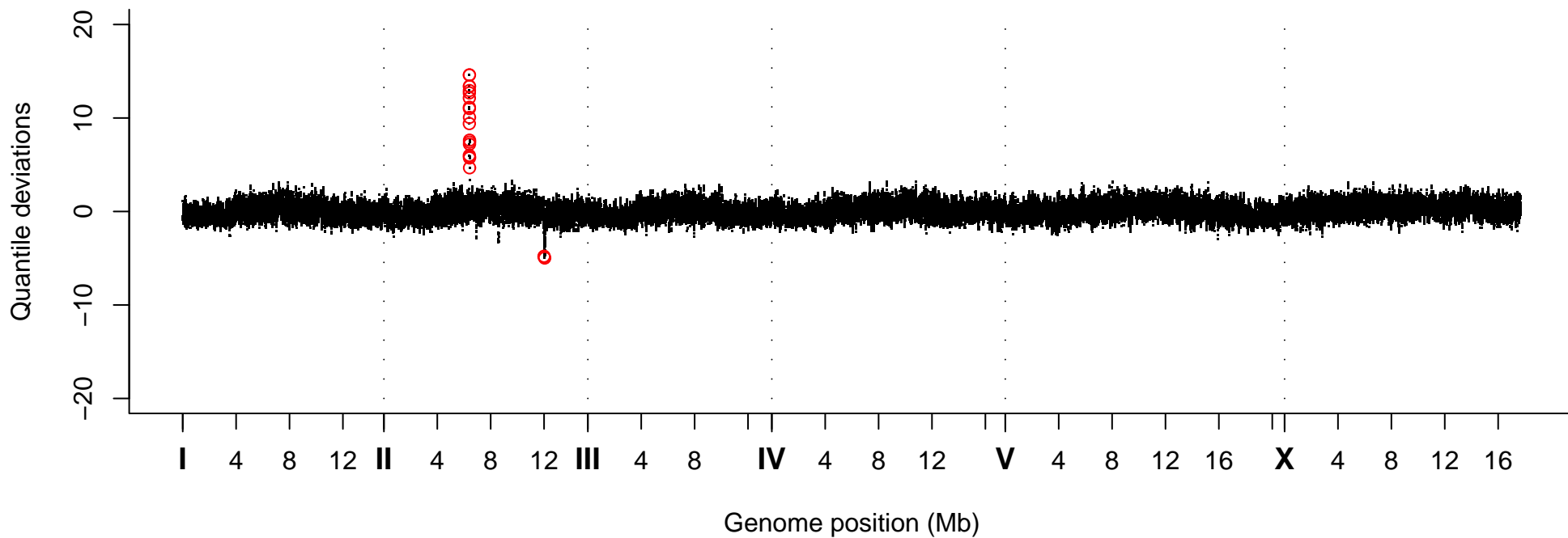
Quantile Deviations, Strain VC40494
