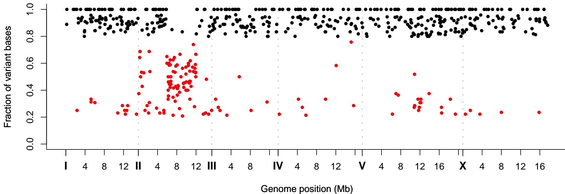
Fraction of Variant Bases at Position, Strain VC40494
