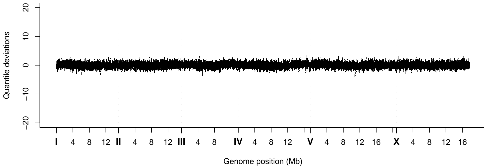
Quantile Deviations, Strain VC40497
