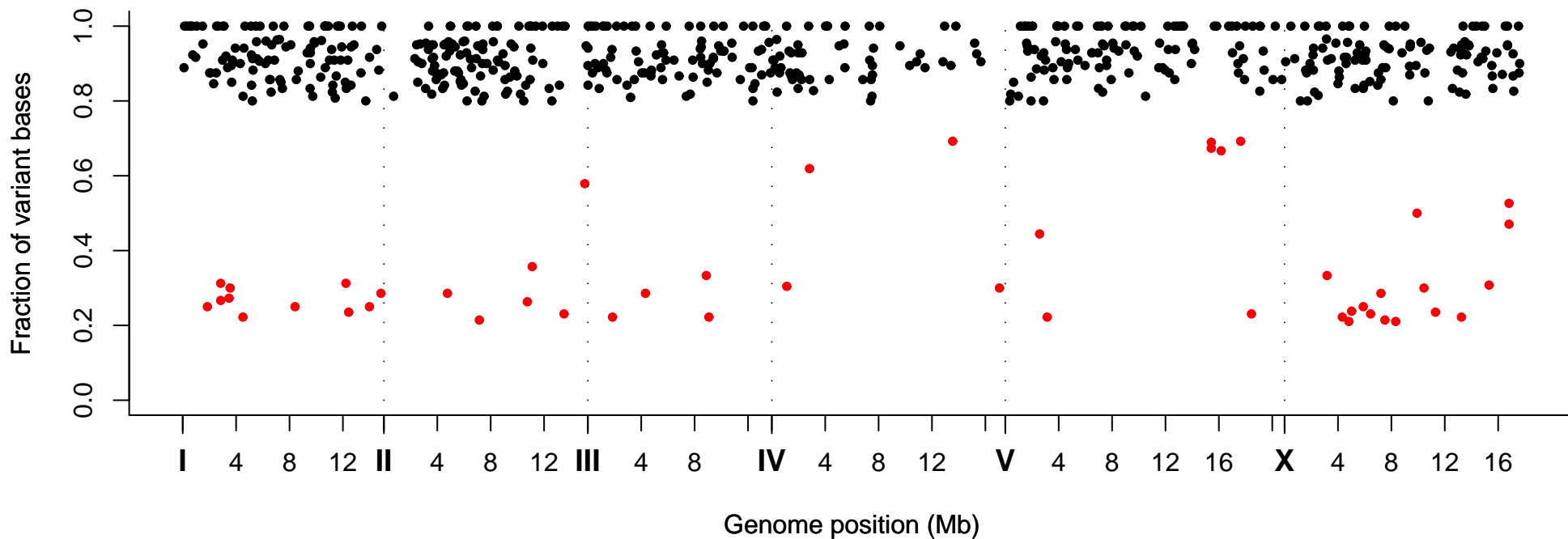
Fraction of Variant Bases at Position, Strain VC40501
