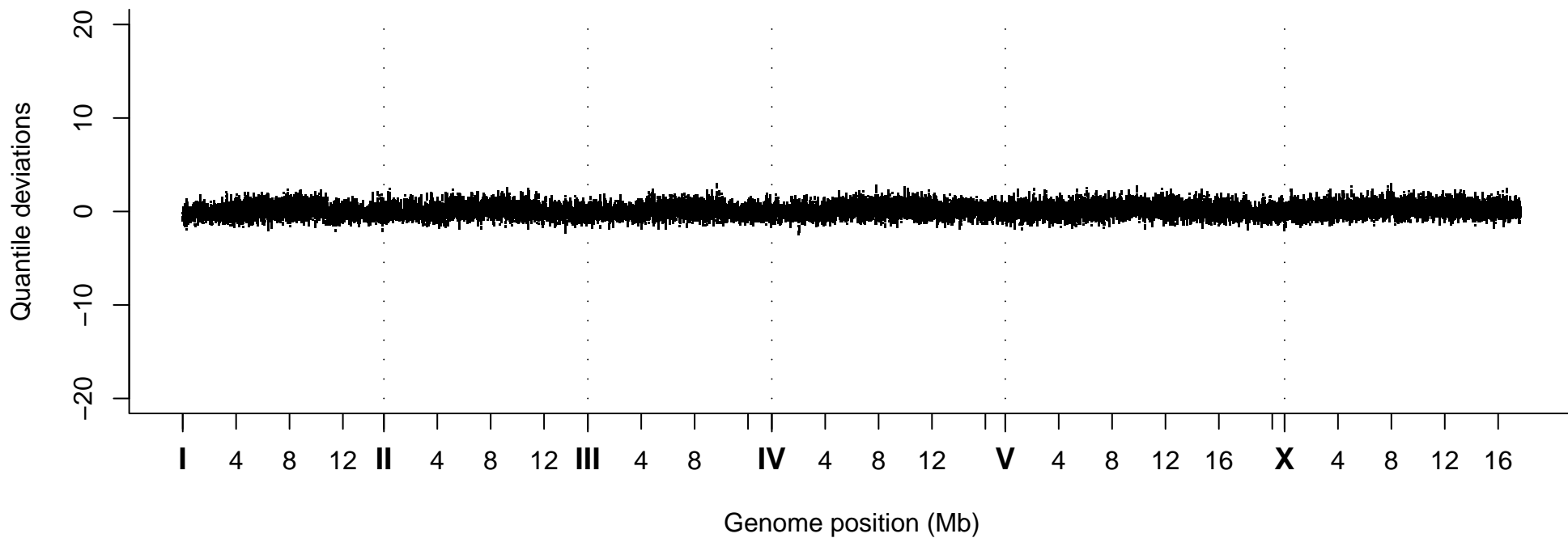
Quantile Deviations, Strain VC40501
