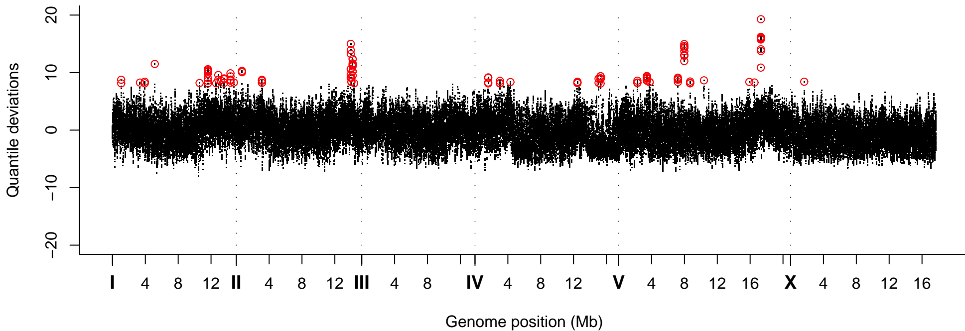
Quantile Deviations, Strain VC40502
