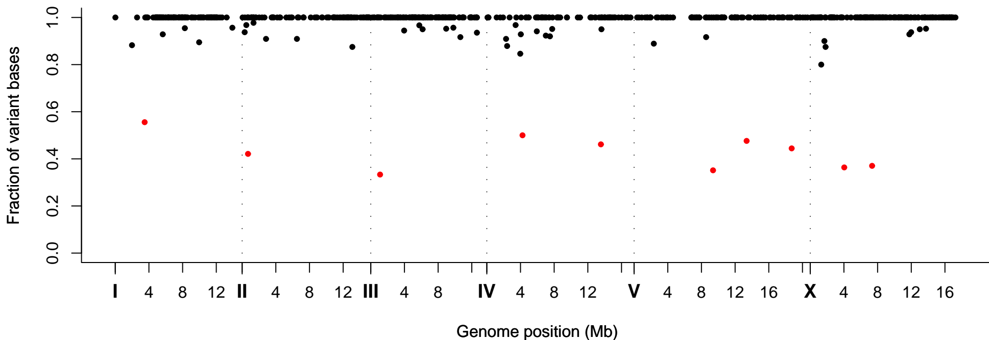
Fraction of Variant Bases at Position, Strain VC40502
