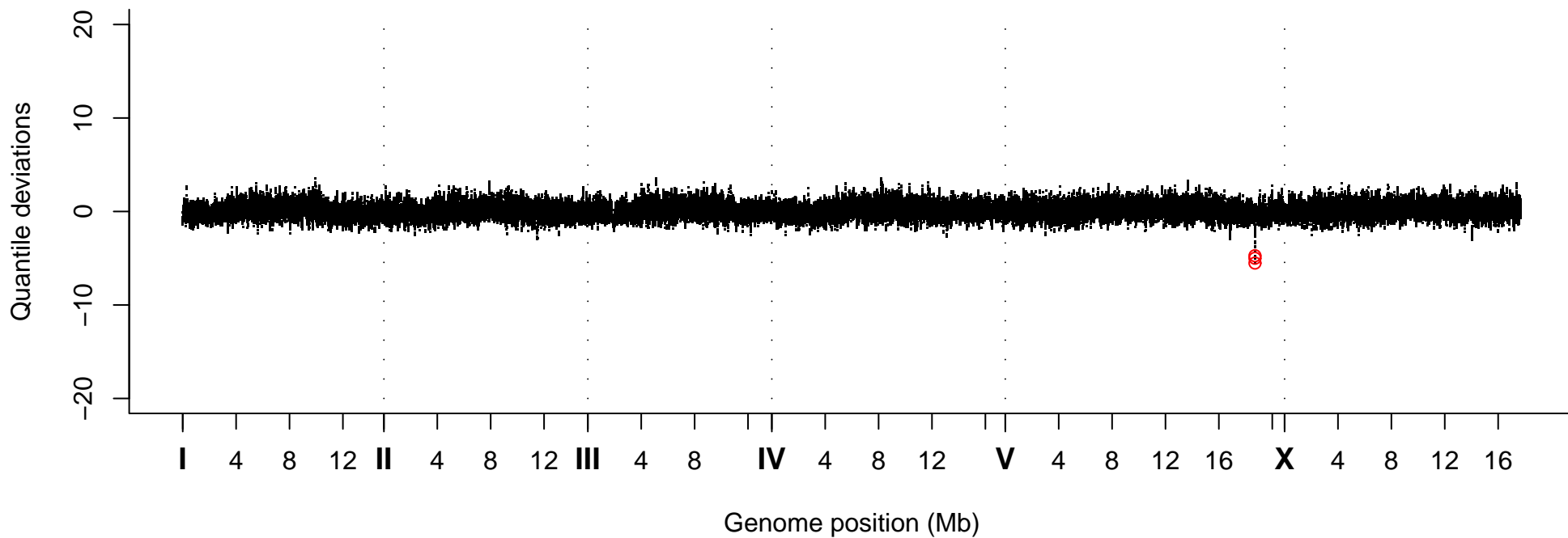
Quantile Deviations, Strain VC40504
