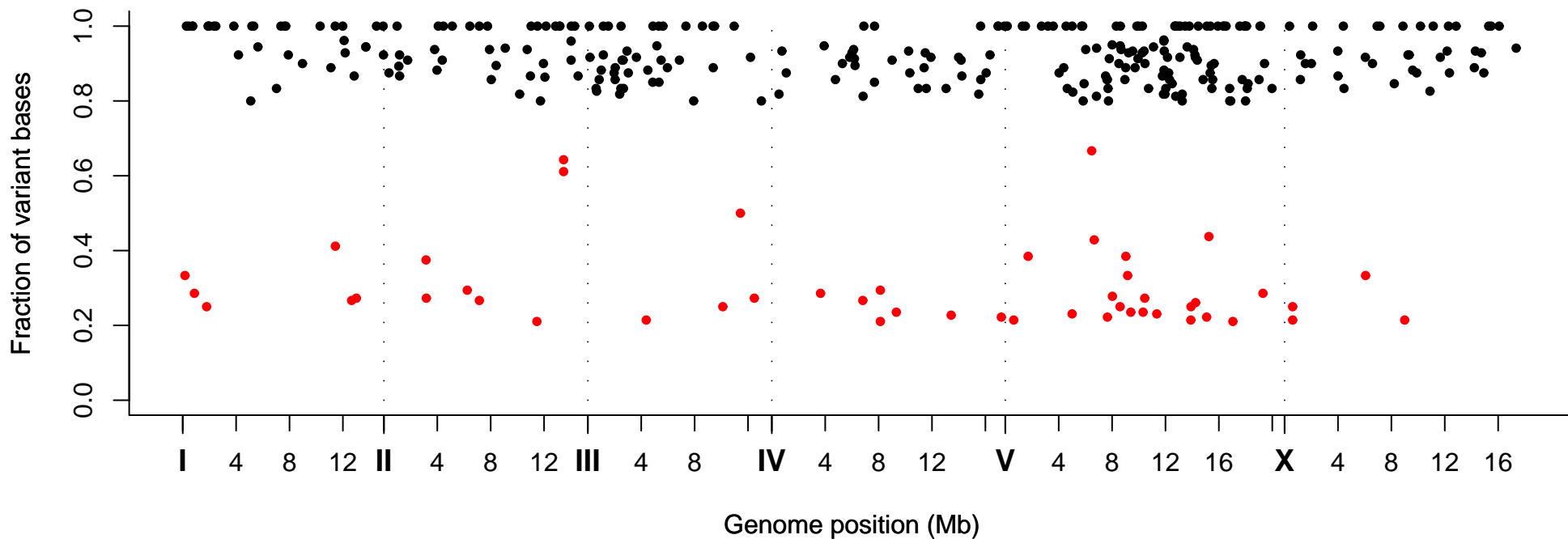
Fraction of Variant Bases at Position, Strain VC40504
