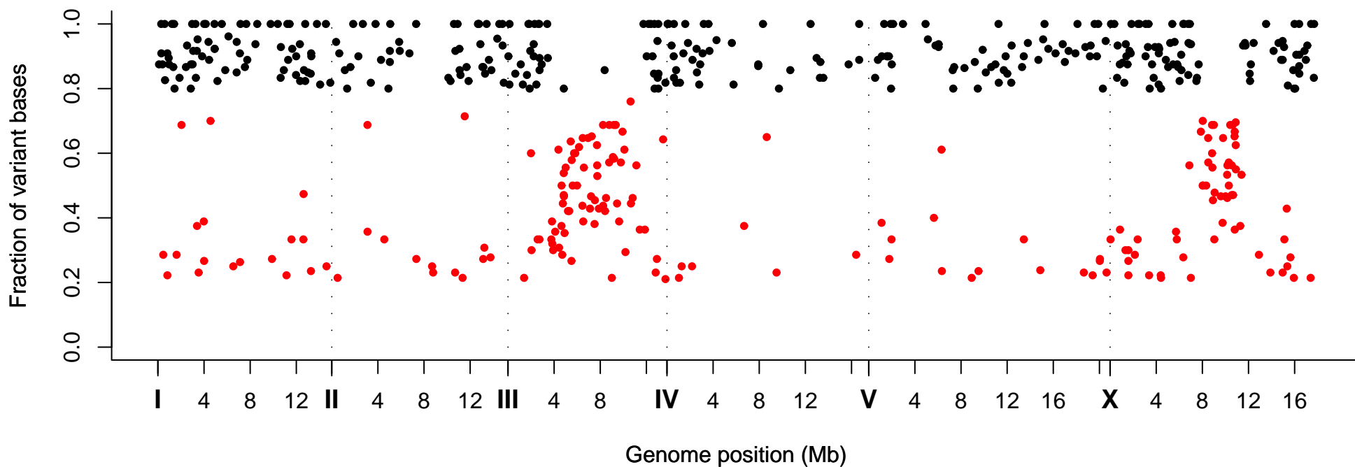
Fraction of Variant Bases at Position, Strain VC40505
