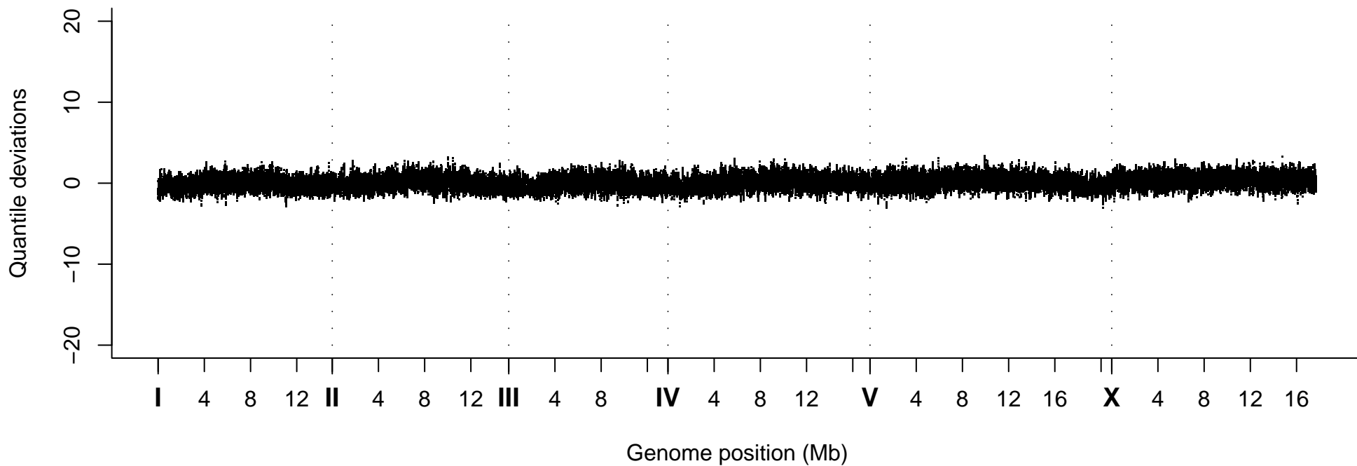
Quantile Deviations, Strain VC40505
