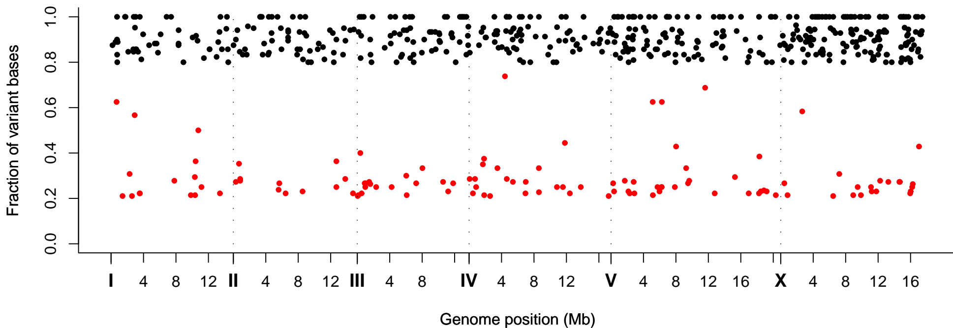
Fraction of Variant Bases at Position, Strain VC40508
