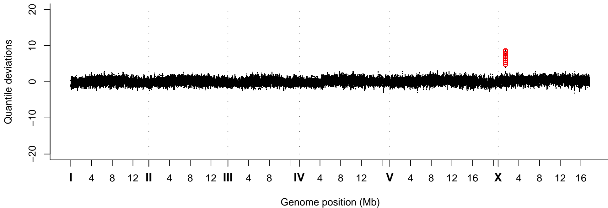
Quantile Deviations, Strain VC40508
