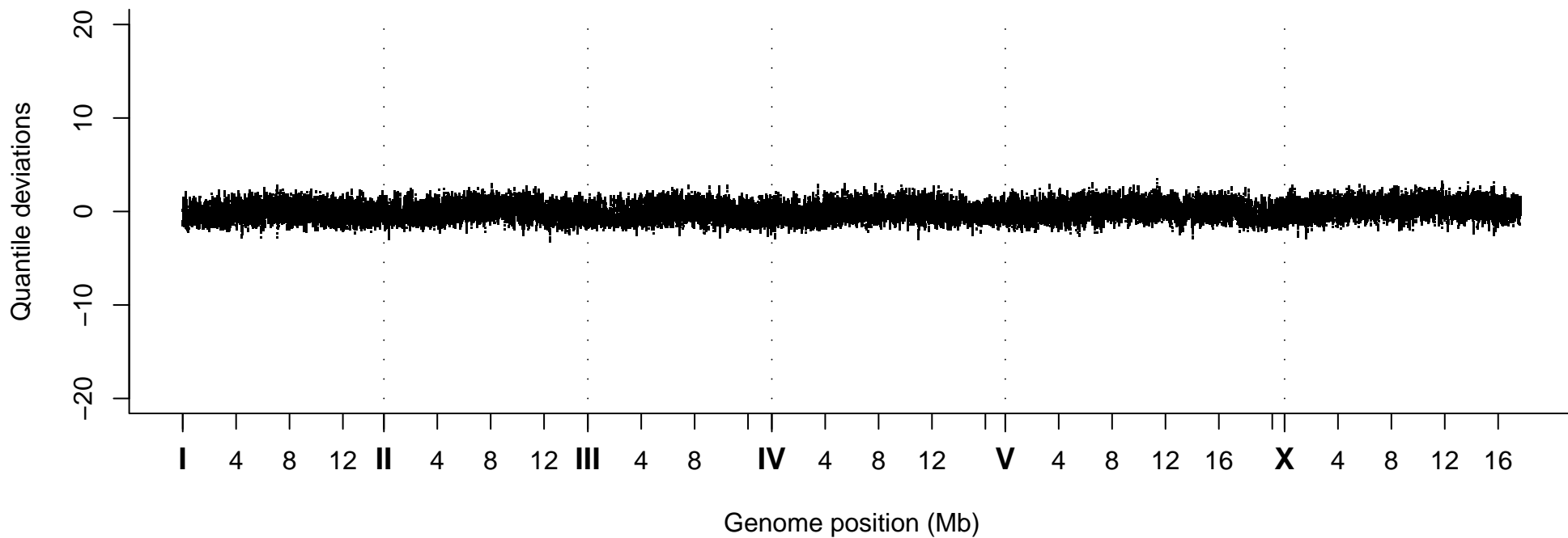
Quantile Deviations, Strain VC40509
