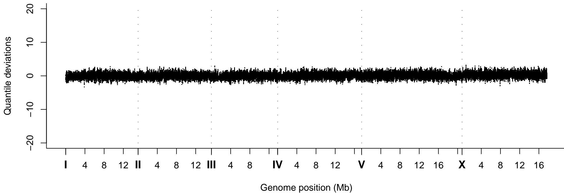
Quantile Deviations, Strain VC40510
