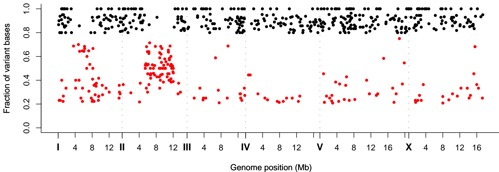
Fraction of Variant Bases at Position, Strain VC40510
