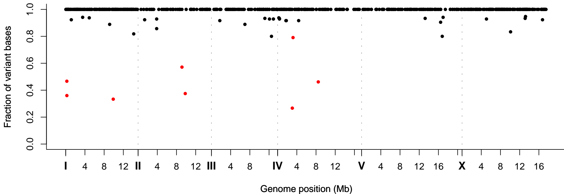
Fraction of Variant Bases at Position, Strain VC40517
