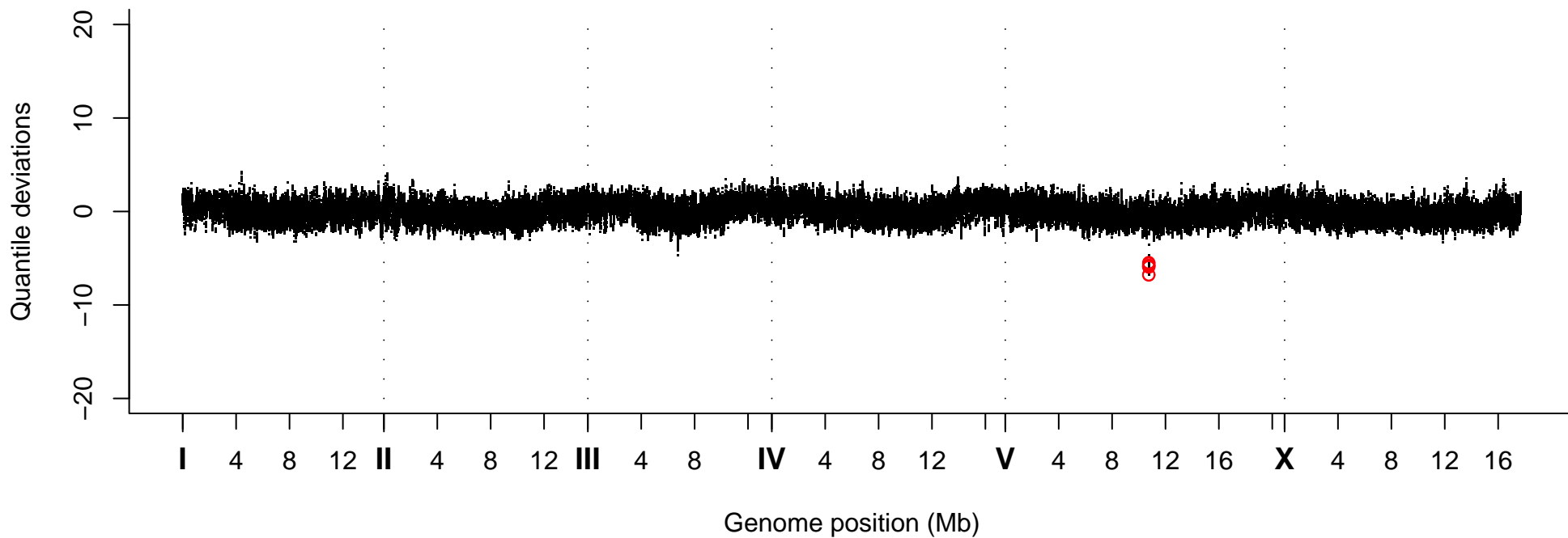
Quantile Deviations, Strain VC40517
