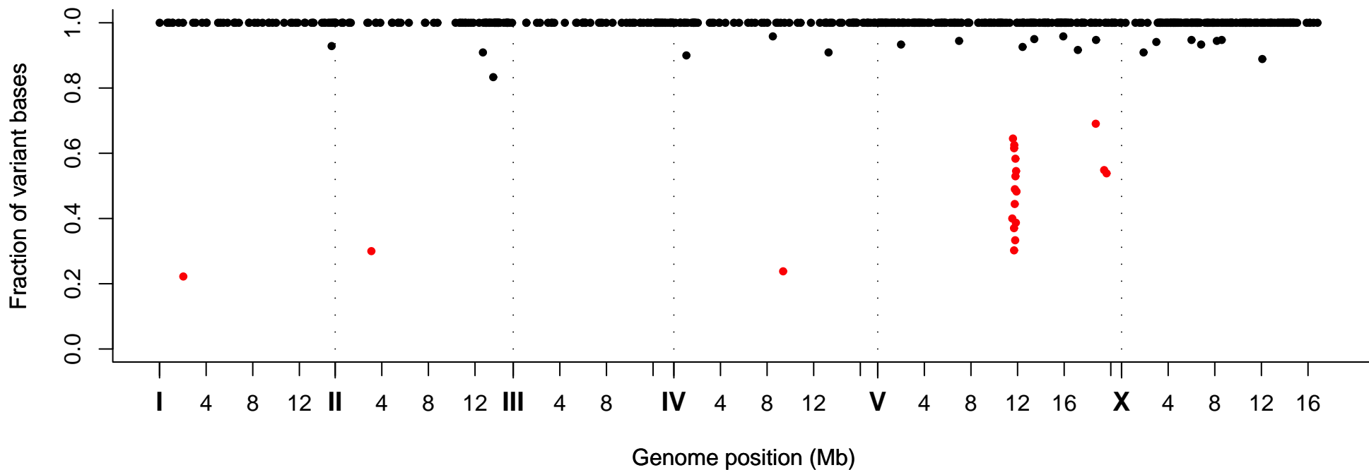
Fraction of Variant Bases at Position, Strain VC40526
