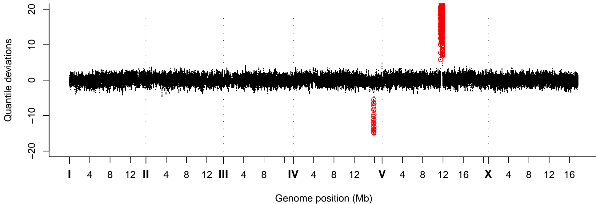
Quantile Deviations, Strain VC40526
