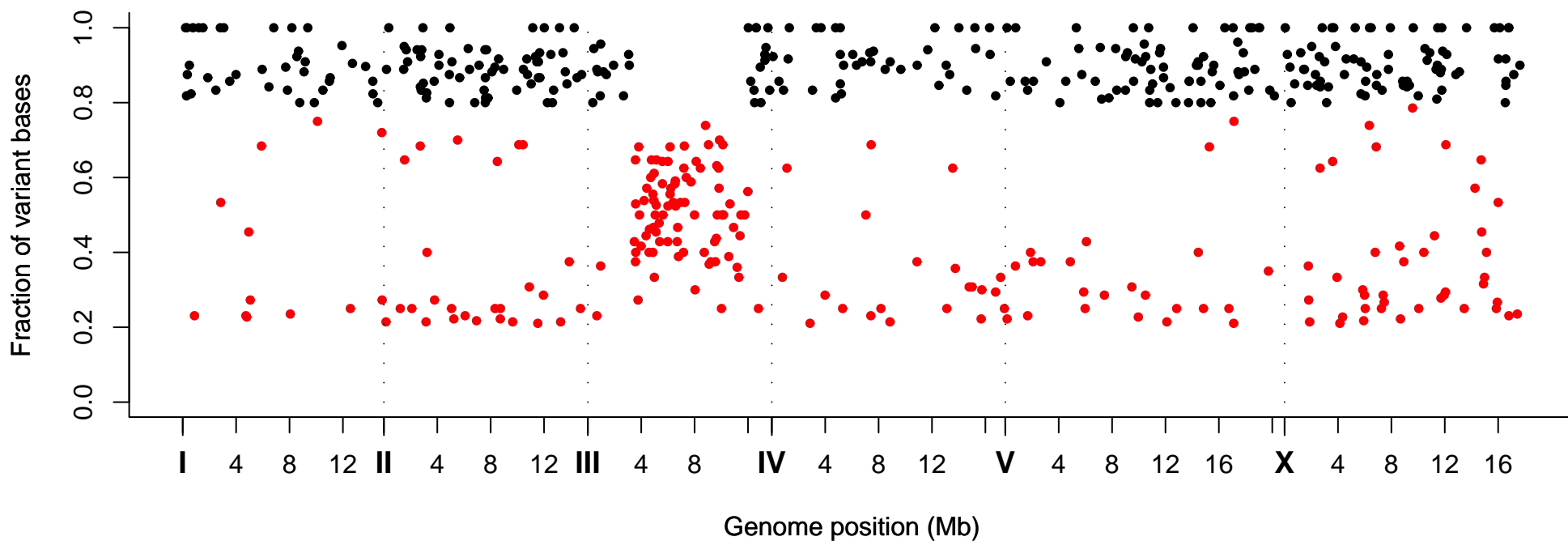
Fraction of Variant Bases at Position, Strain VC40528
