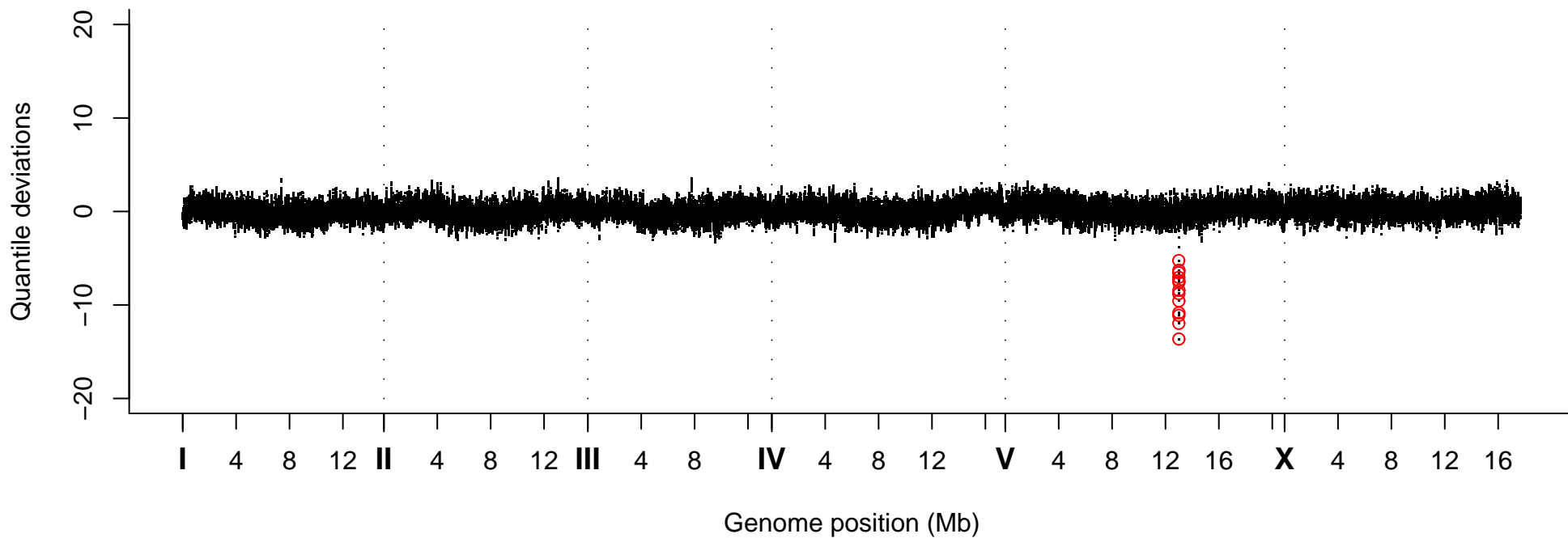
Quantile Deviations, Strain VC40528
