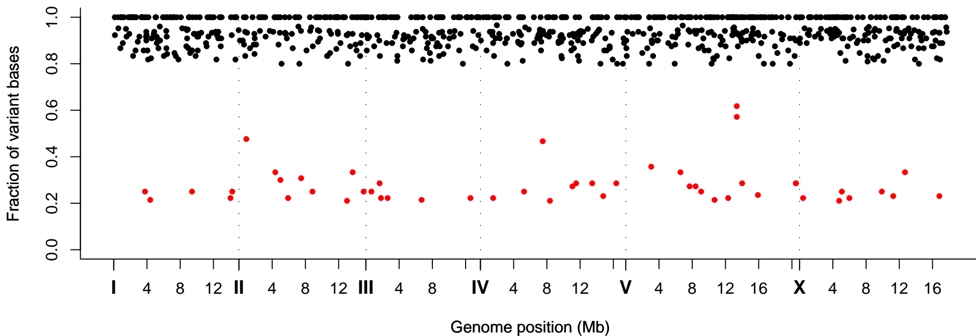
Fraction of Variant Bases at Position, Strain VC40532
