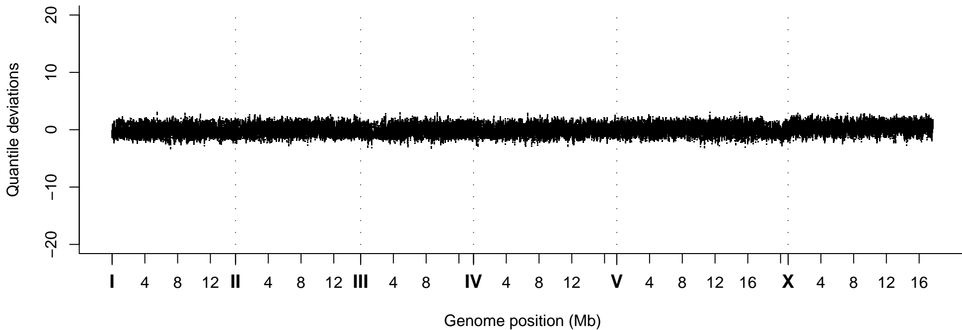
Quantile Deviations, Strain VC40532
