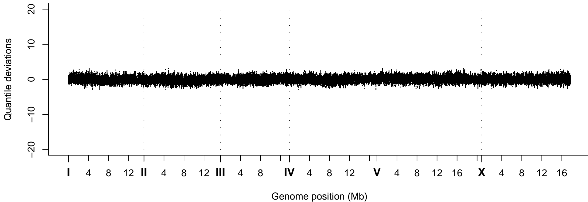
Quantile Deviations, Strain VC40538
