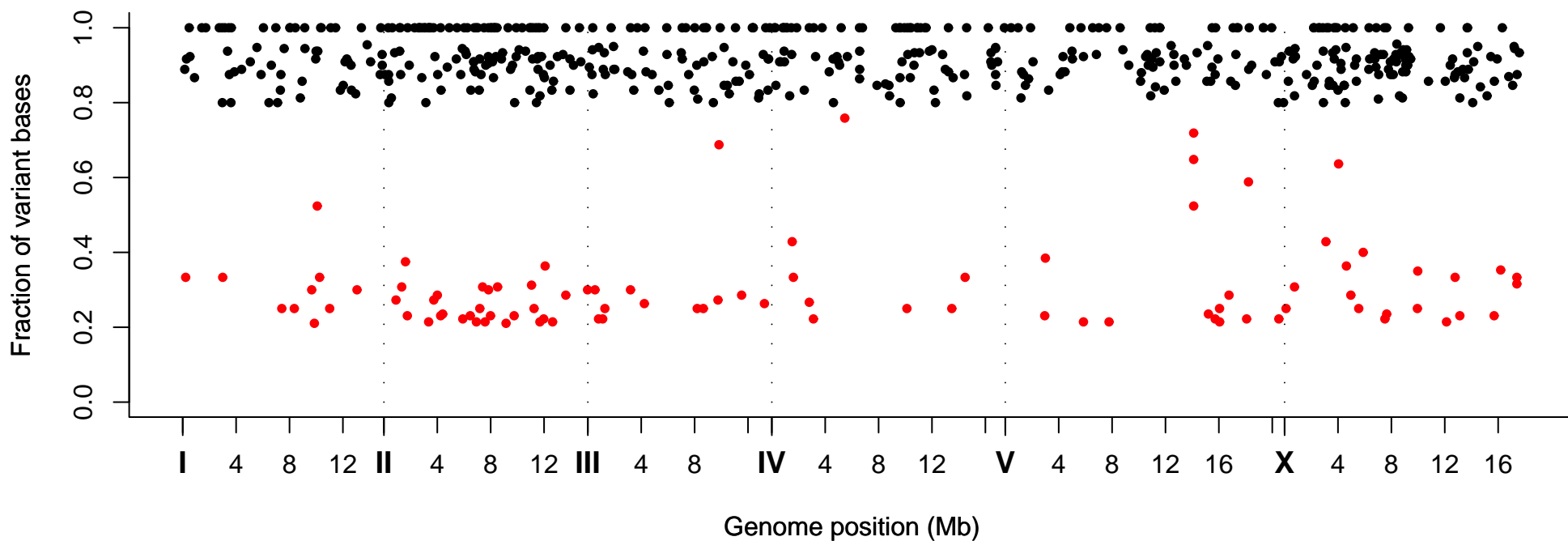
Fraction of Variant Bases at Position, Strain VC40538
