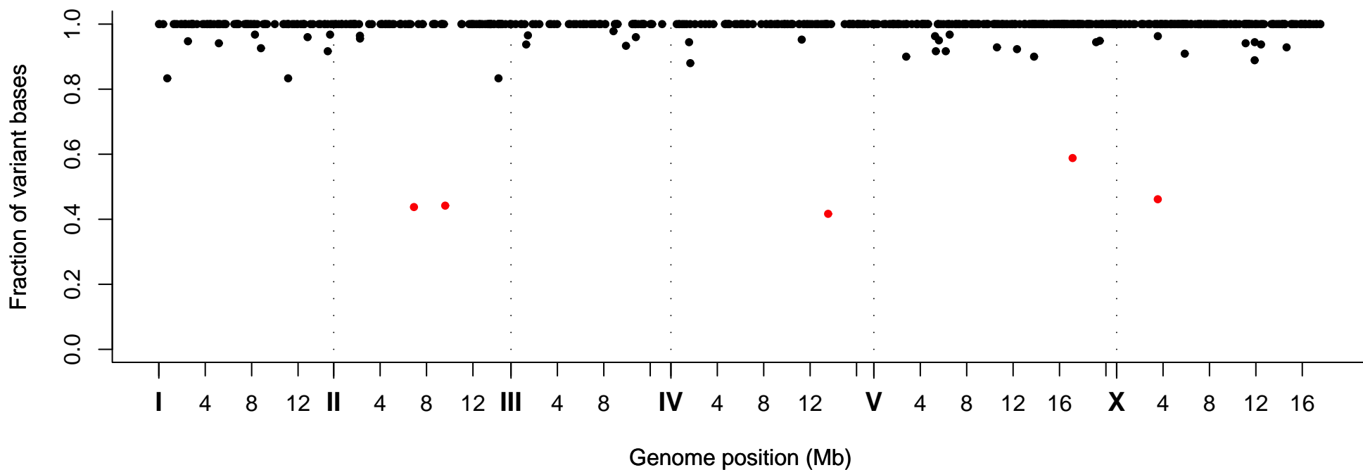
Fraction of Variant Bases at Position, Strain VC40542
