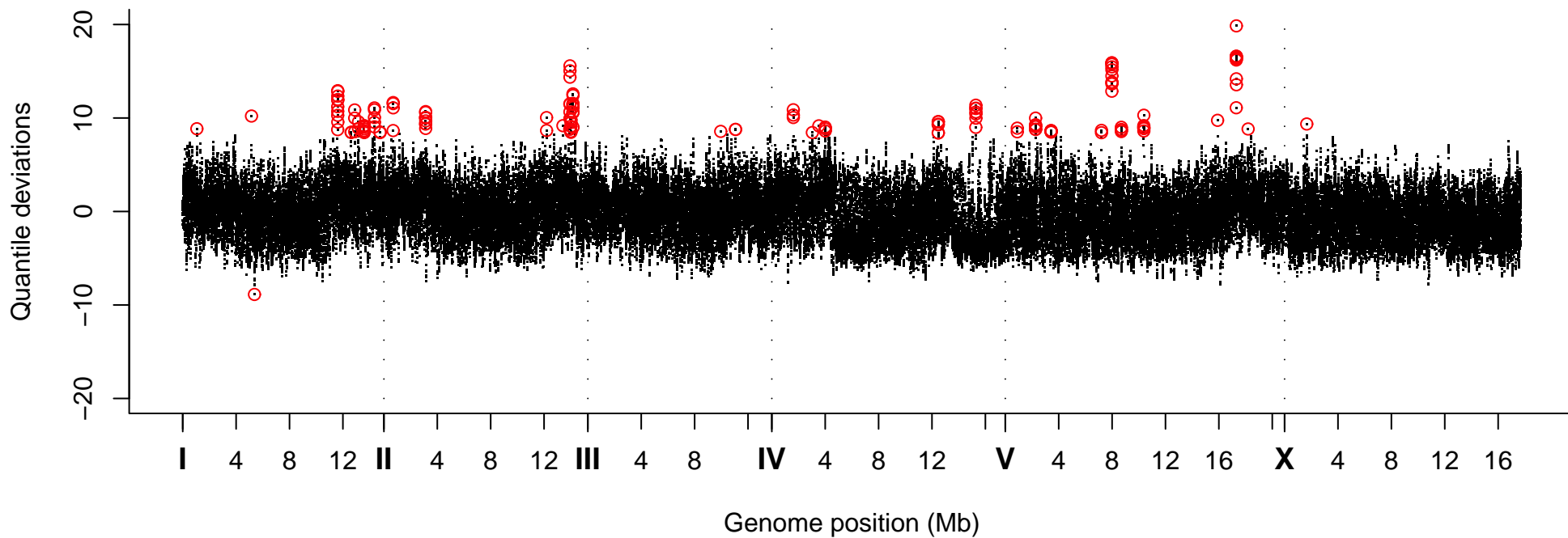
Quantile Deviations, Strain VC40542
