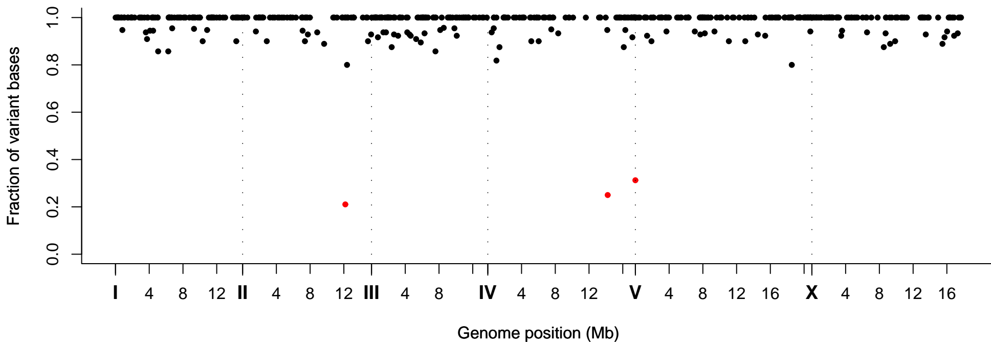
Fraction of Variant Bases at Position, Strain VC40549
