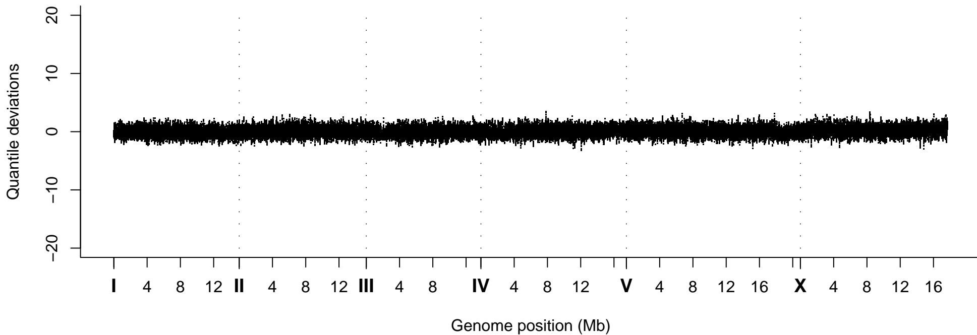
Quantile Deviations, Strain VC40549
