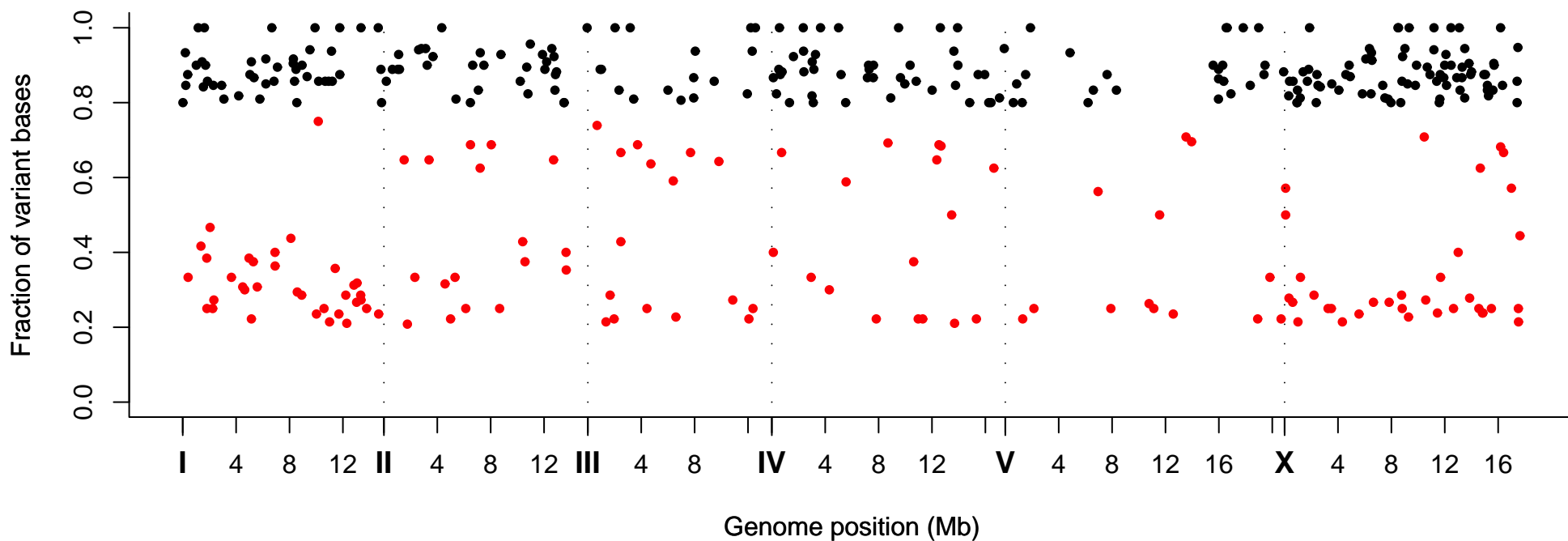
Fraction of Variant Bases at Position, Strain VC40550
