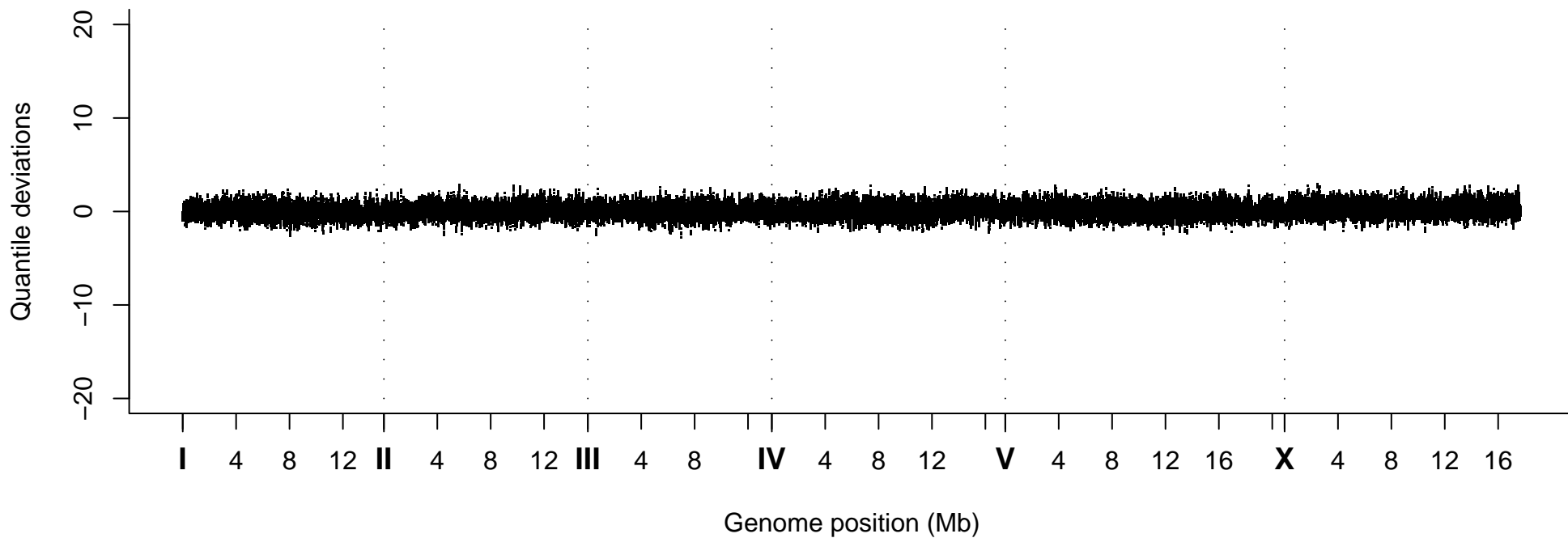
Quantile Deviations, Strain VC40550
