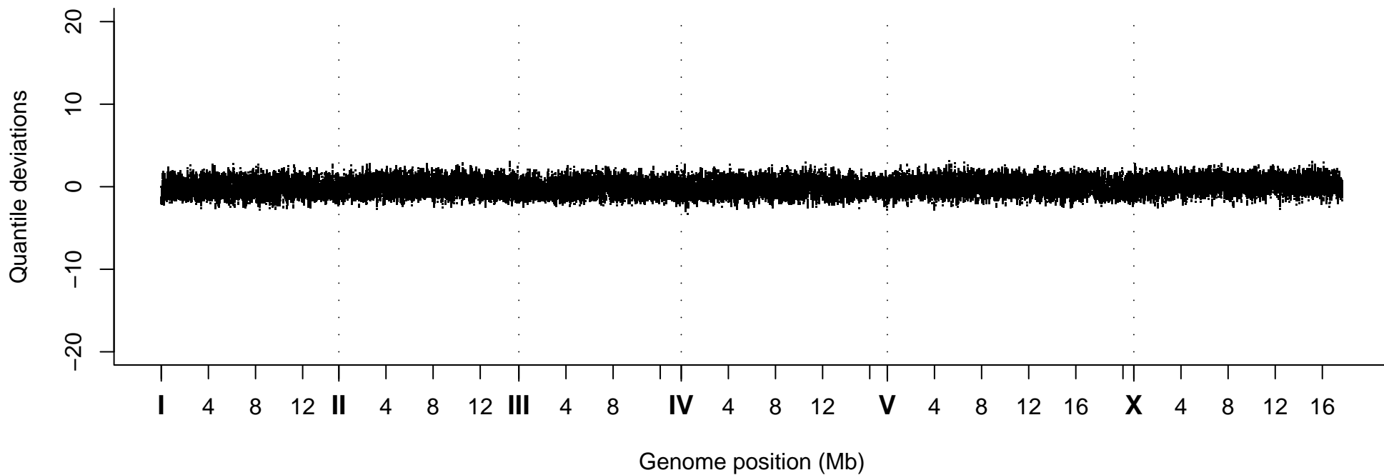
Quantile Deviations, Strain VC40554
