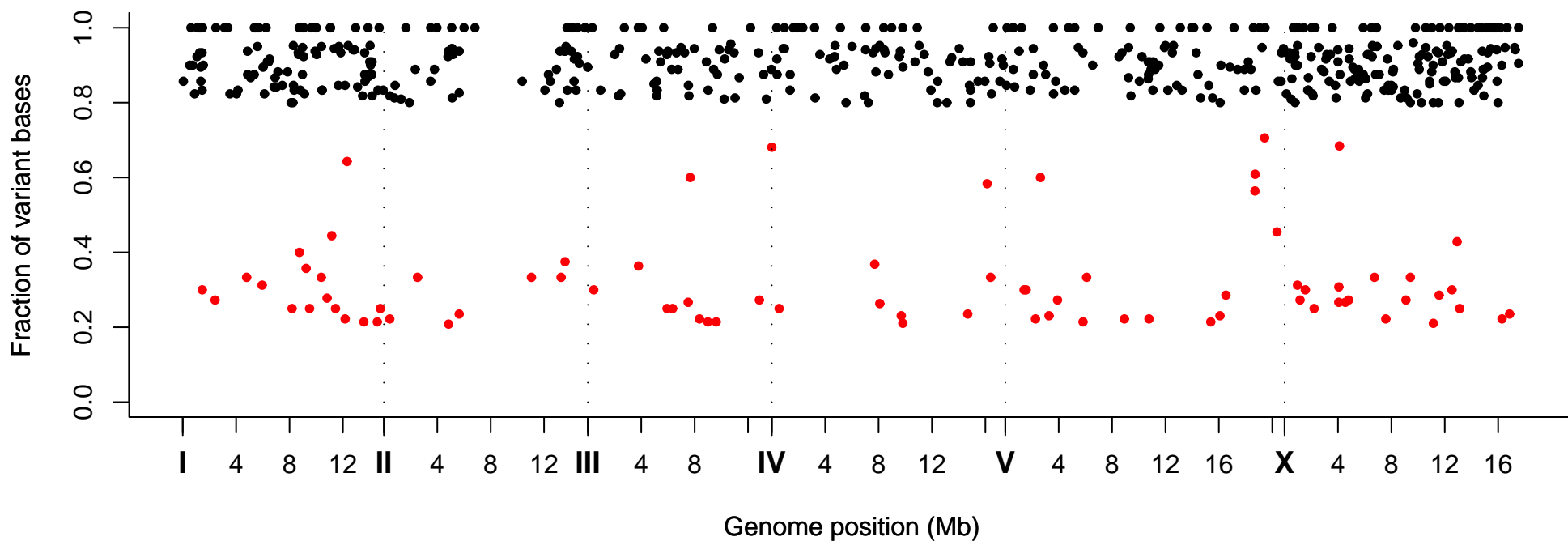
Fraction of Variant Bases at Position, Strain VC40554
