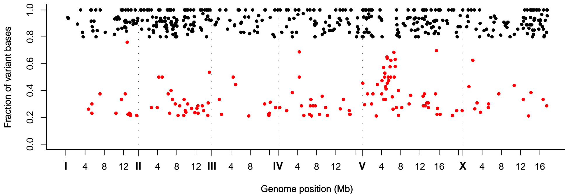
Fraction of Variant Bases at Position, Strain VC40555
