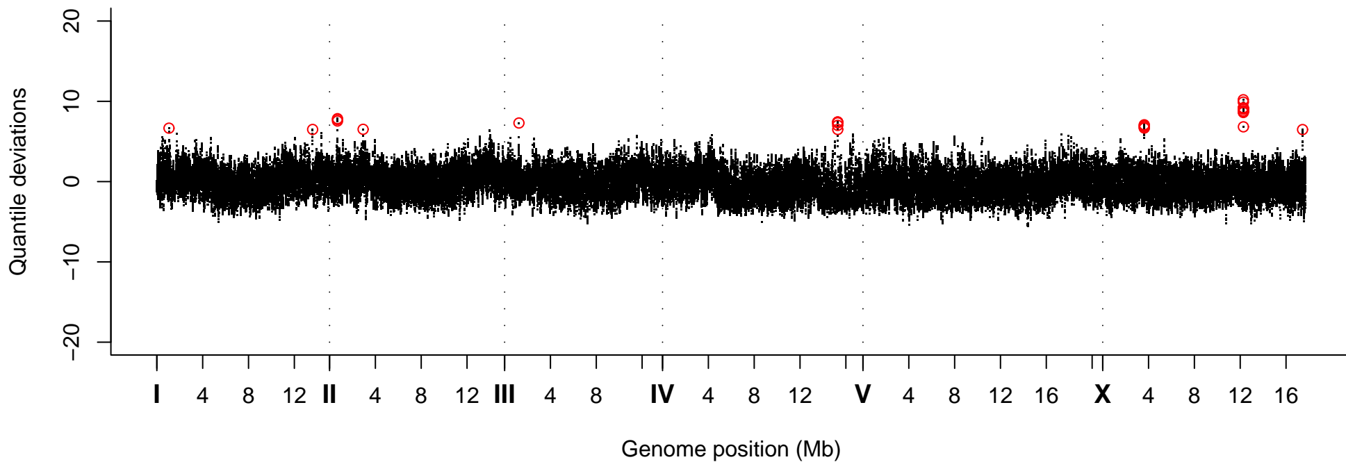
Quantile Deviations, Strain VC40555
