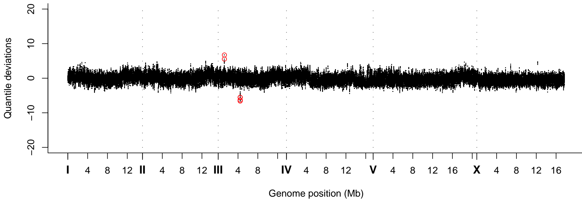
Quantile Deviations, Strain VC40558
