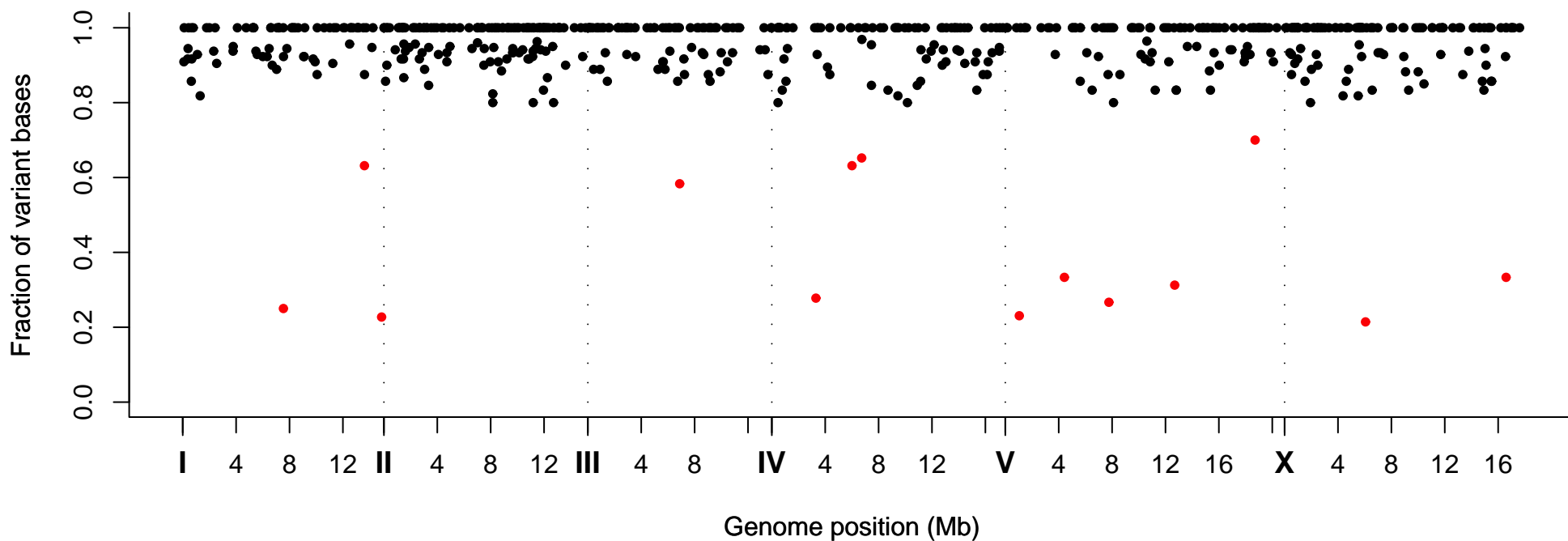
Fraction of Variant Bases at Position, Strain VC40558
