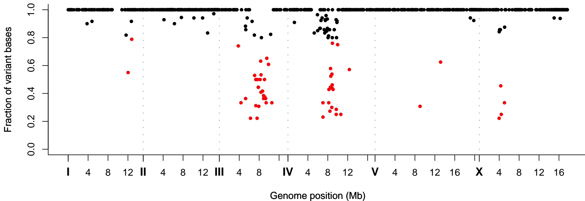
Fraction of Variant Bases at Position, Strain VC40560
