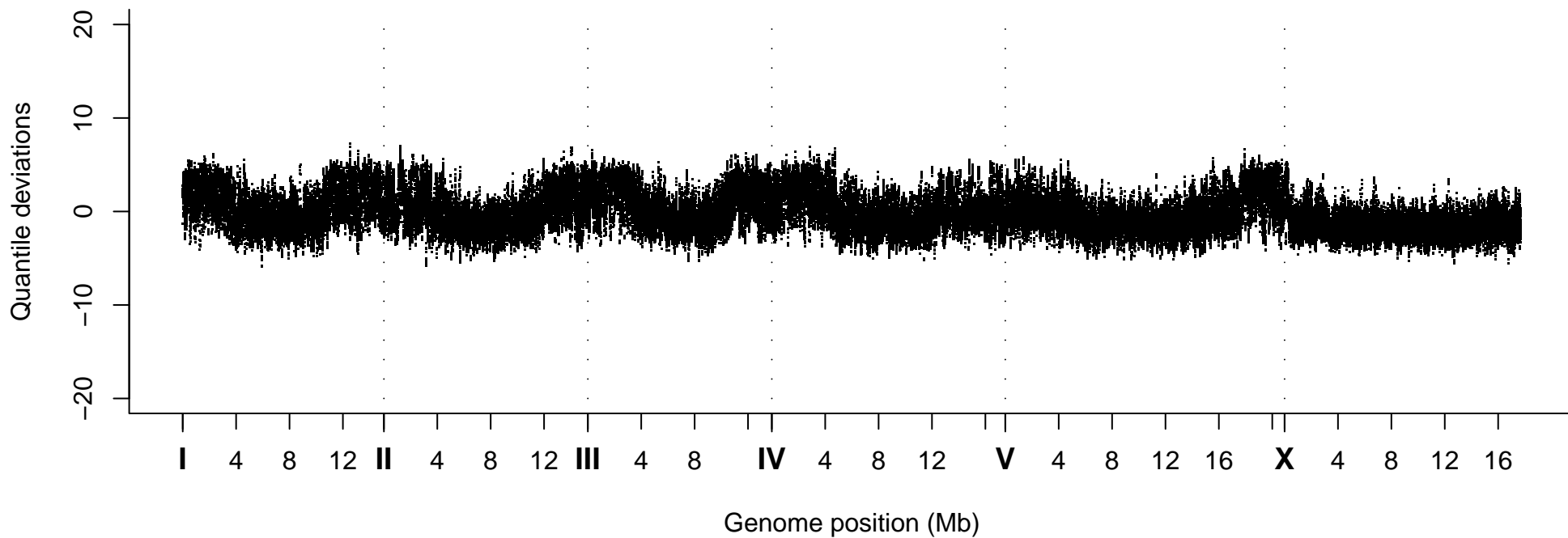
Quantile Deviations, Strain VC40560
