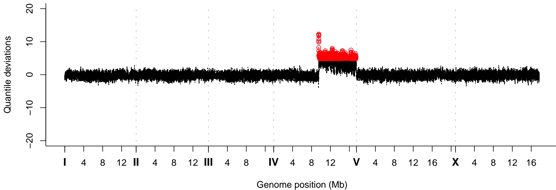
Quantile Deviations, Strain VC40561
