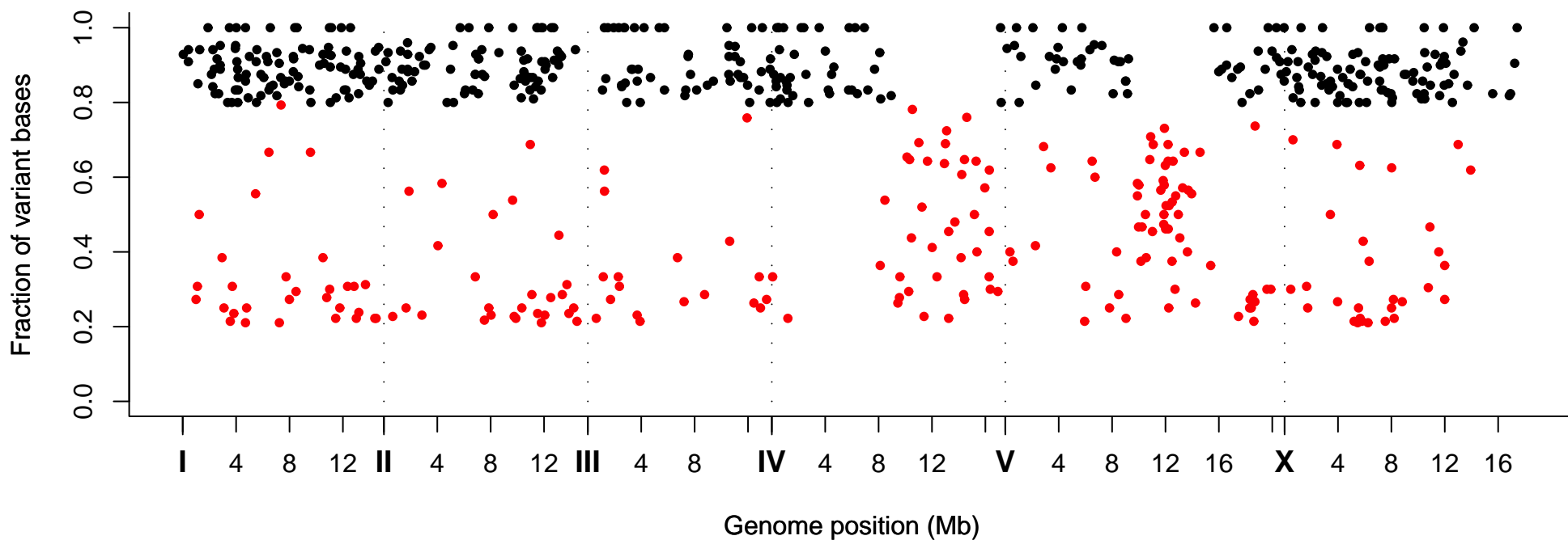
Fraction of Variant Bases at Position, Strain VC40561
