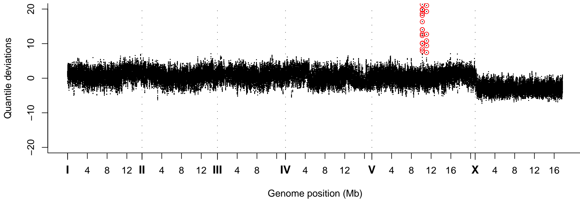
Quantile Deviations, Strain VC40562
