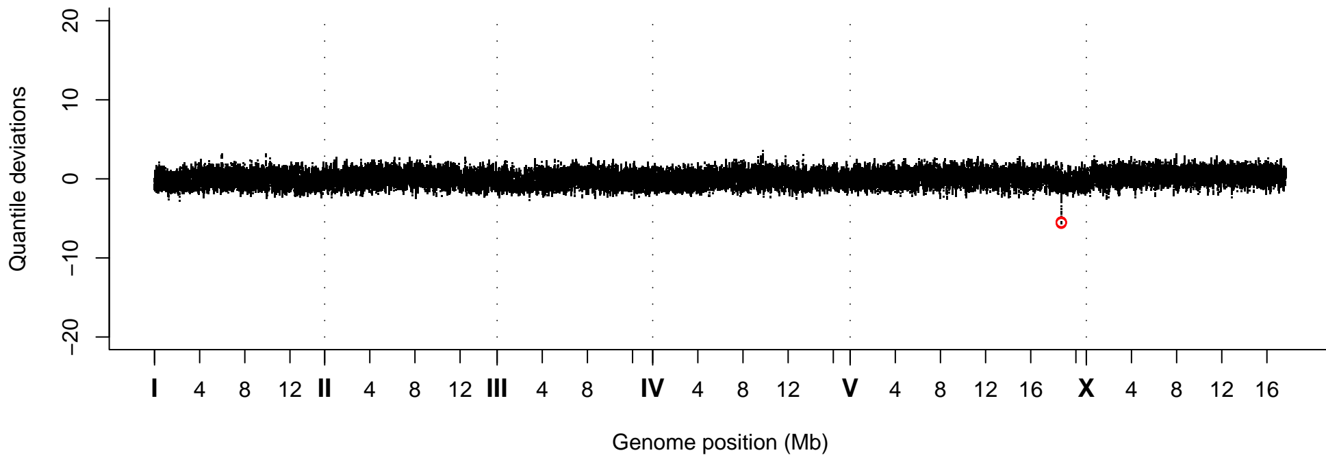
Quantile Deviations, Strain VC40564
