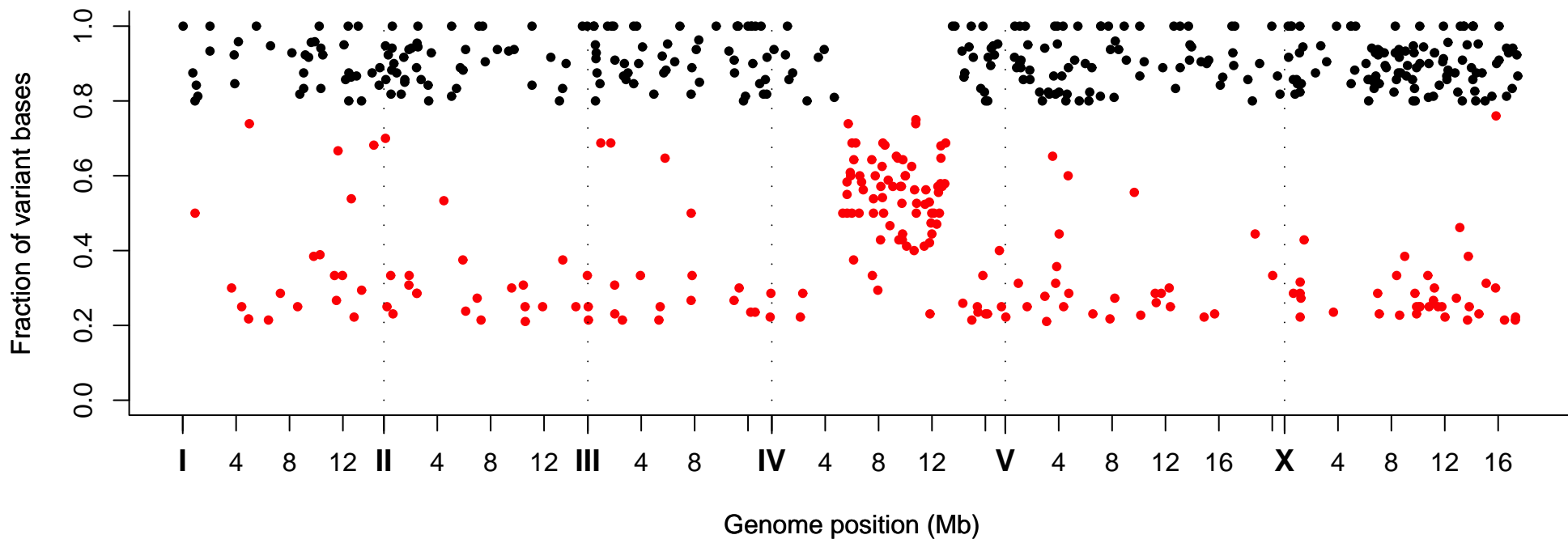
Fraction of Variant Bases at Position, Strain VC40564
