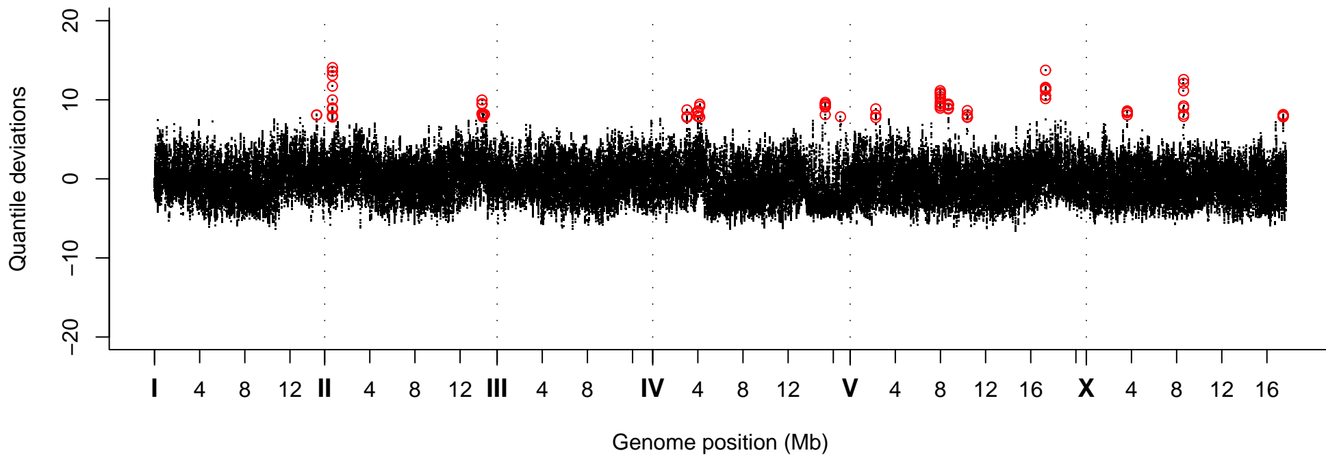
Quantile Deviations, Strain VC40568
