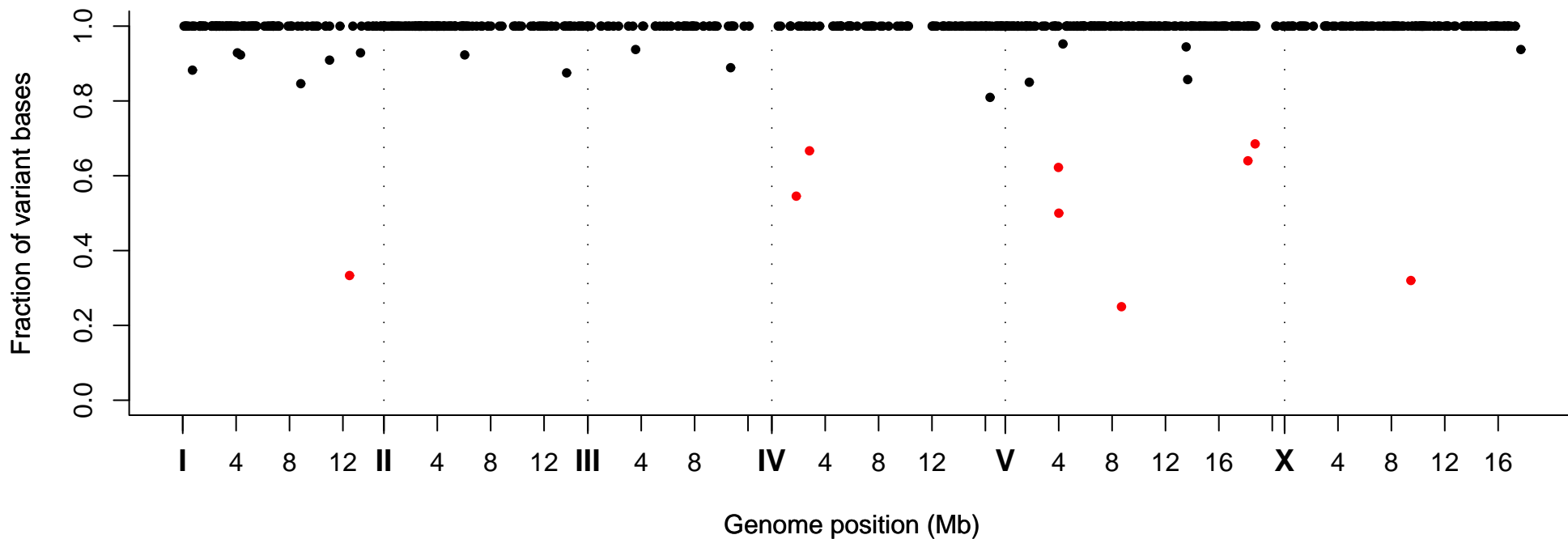
Fraction of Variant Bases at Position, Strain VC40572
