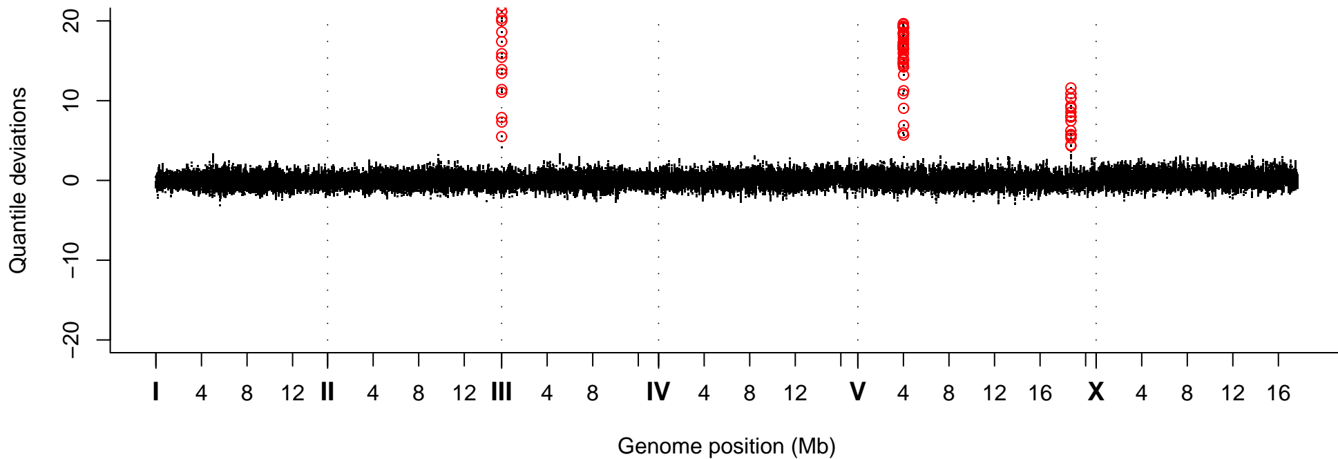
Quantile Deviations, Strain VC40572
