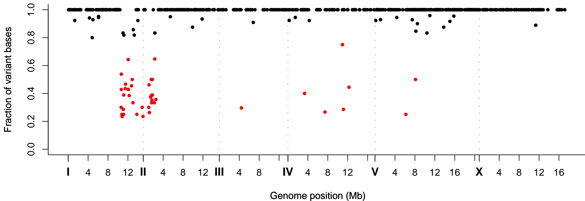
Fraction of Variant Bases at Position, Strain VC40574
