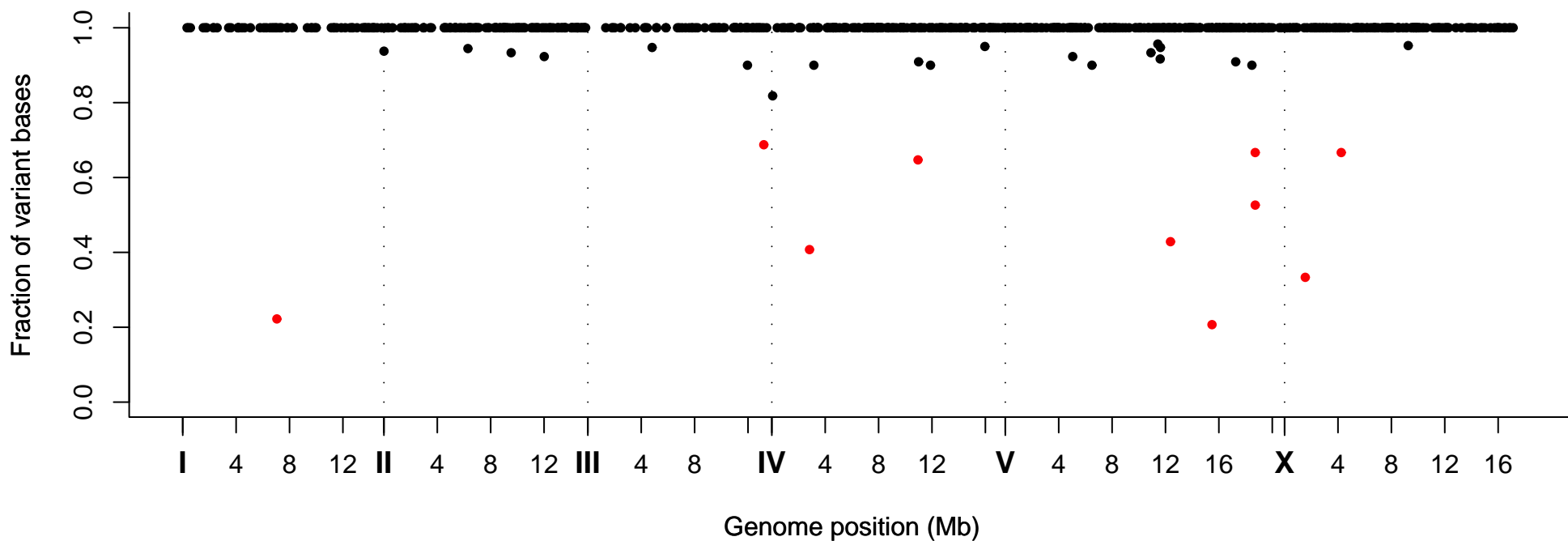
Fraction of Variant Bases at Position, Strain VC40576
