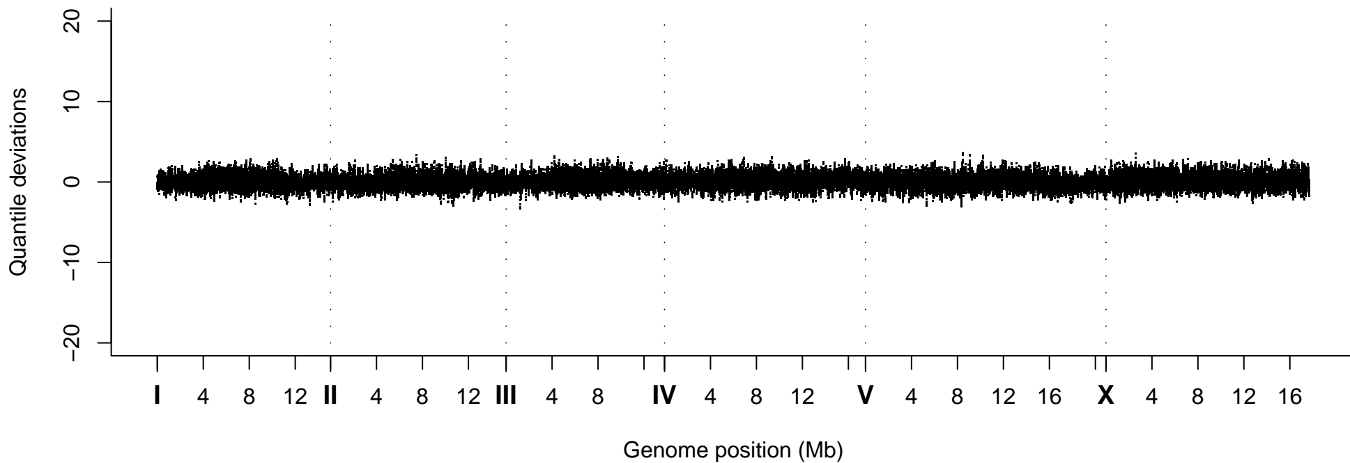
Quantile Deviations, Strain VC40576
