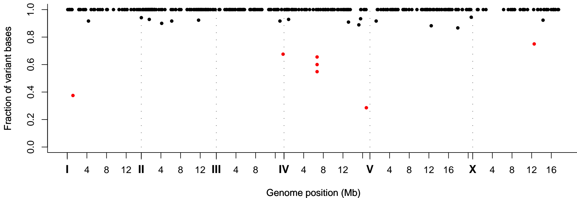
Fraction of Variant Bases at Position, Strain VC40578
