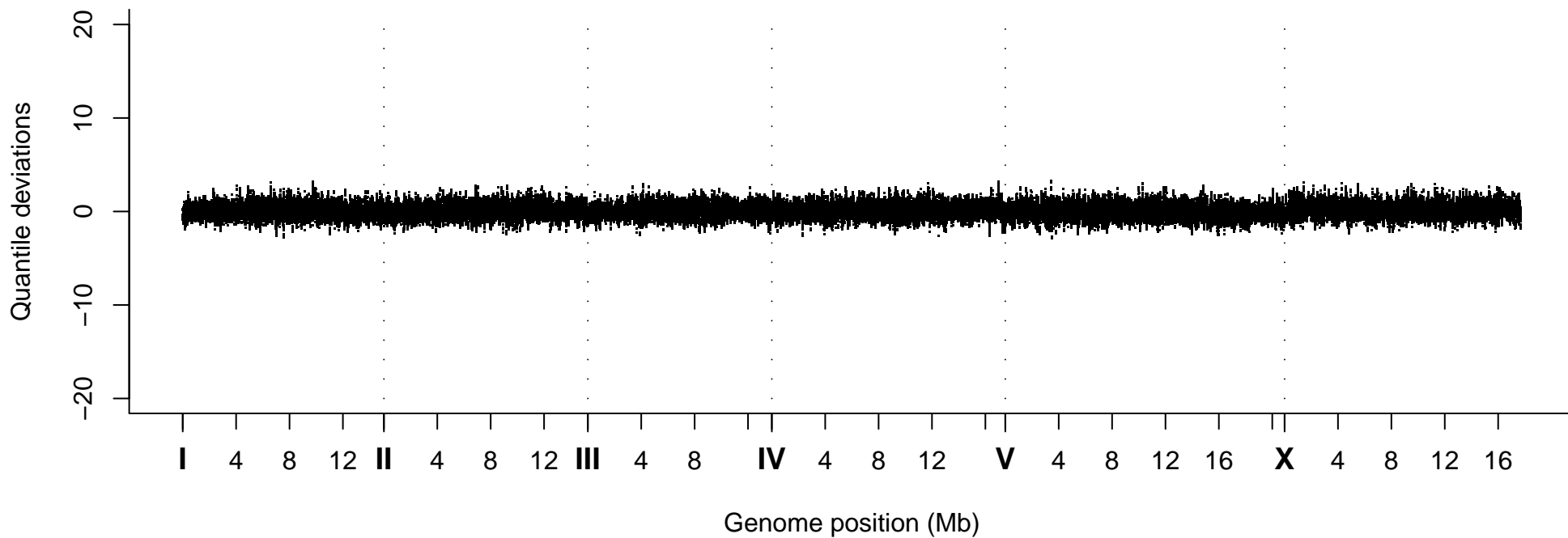
Quantile Deviations, Strain VC40578
