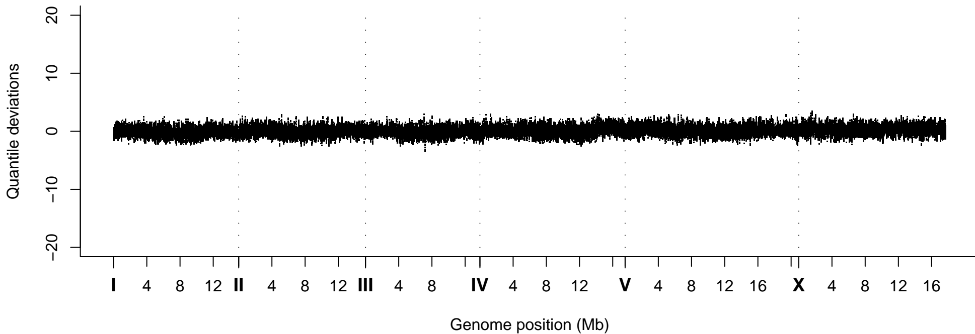
Quantile Deviations, Strain VC40596
