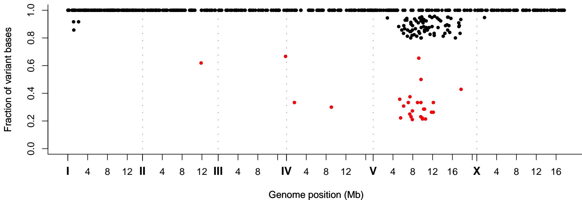
Fraction of Variant Bases at Position, Strain VC40596
