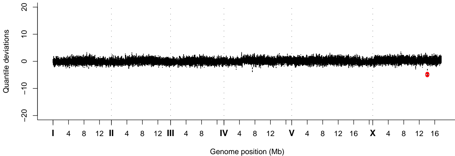
Quantile Deviations, Strain VC40601
