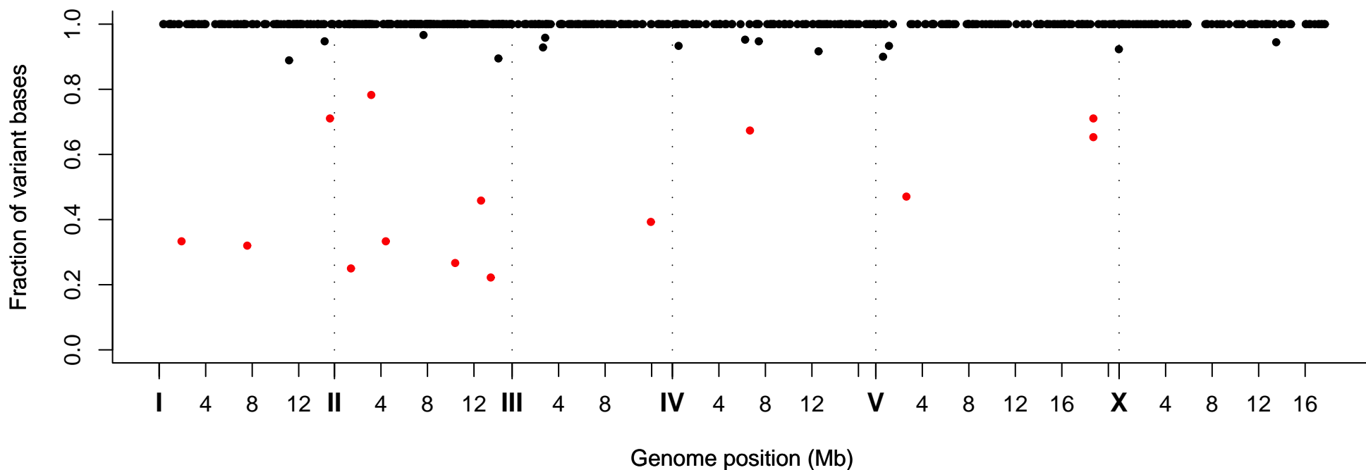
Fraction of Variant Bases at Position, Strain VC40601
