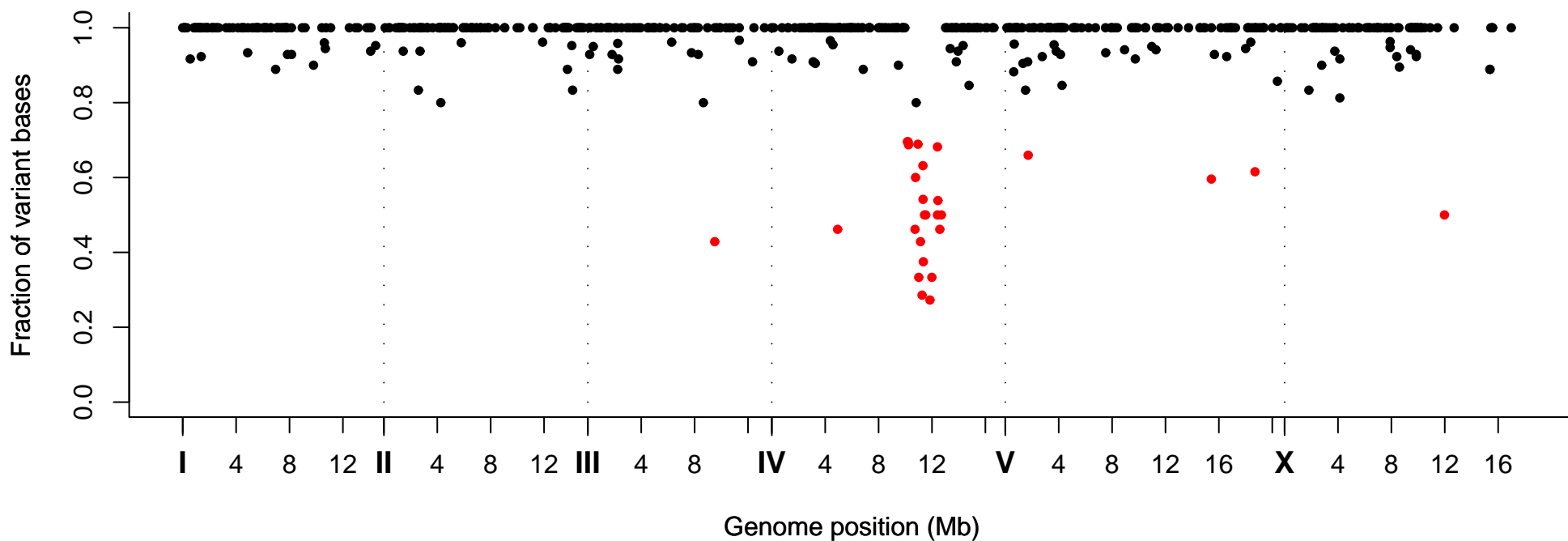
Fraction of Variant Bases at Position, Strain VC40603
