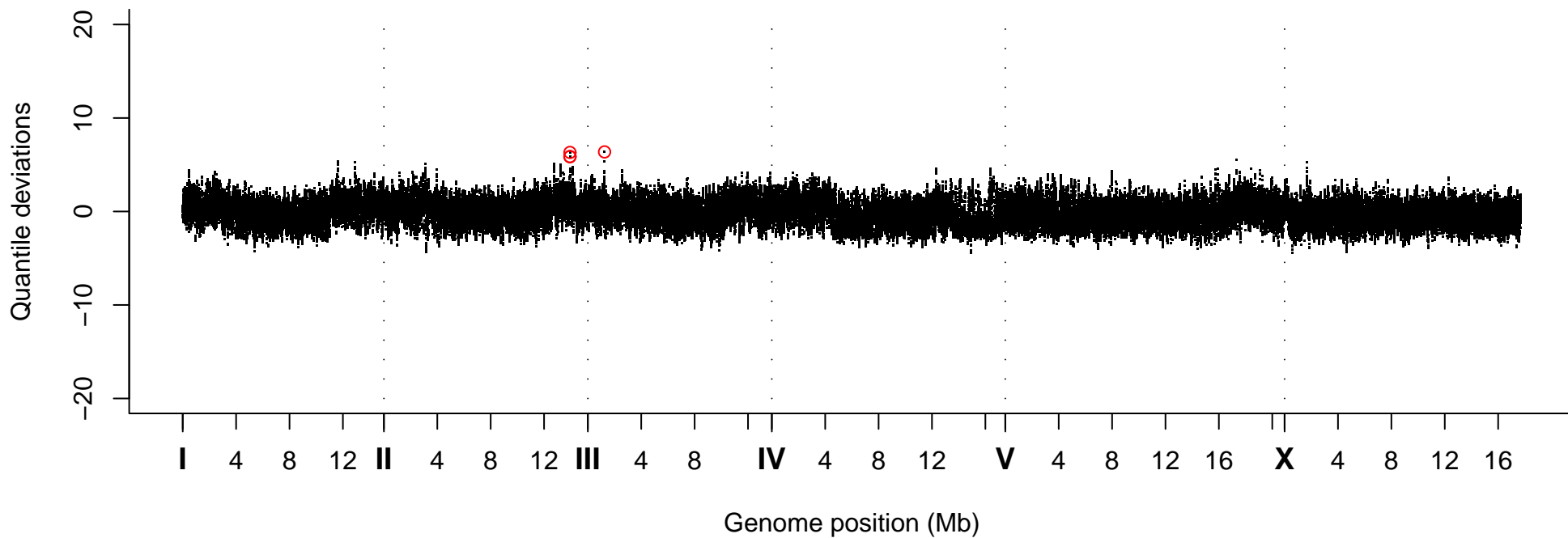
Quantile Deviations, Strain VC40603
