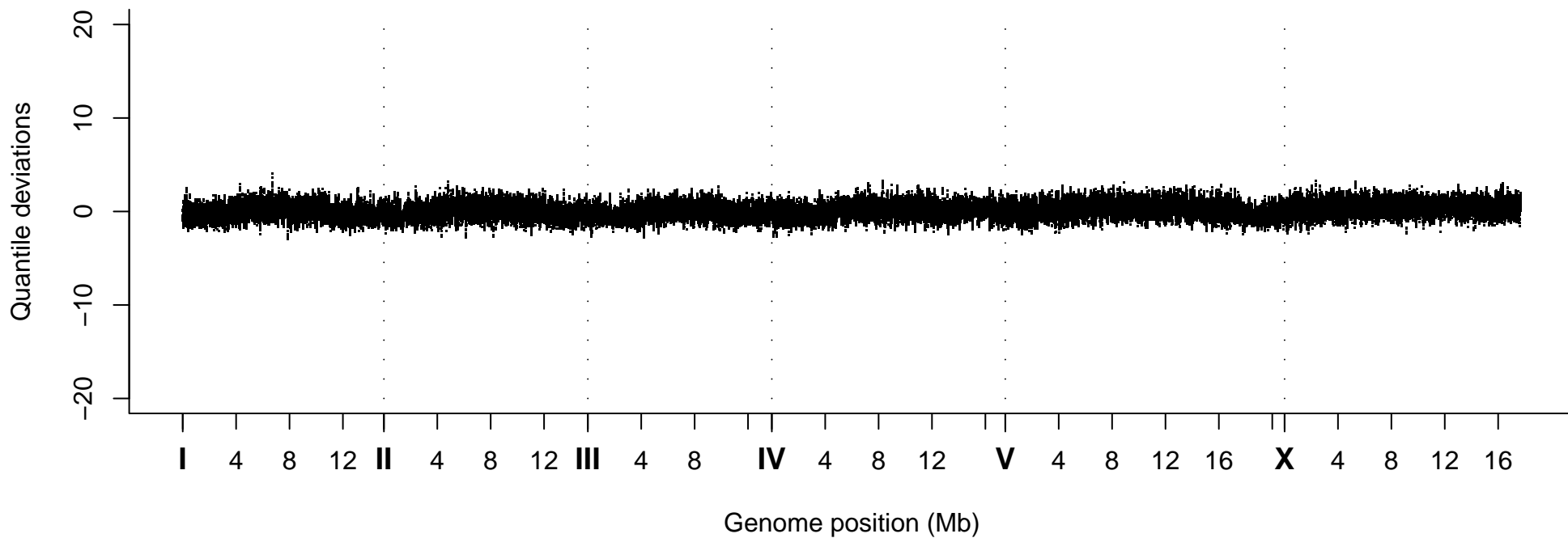
Quantile Deviations, Strain VC40607
