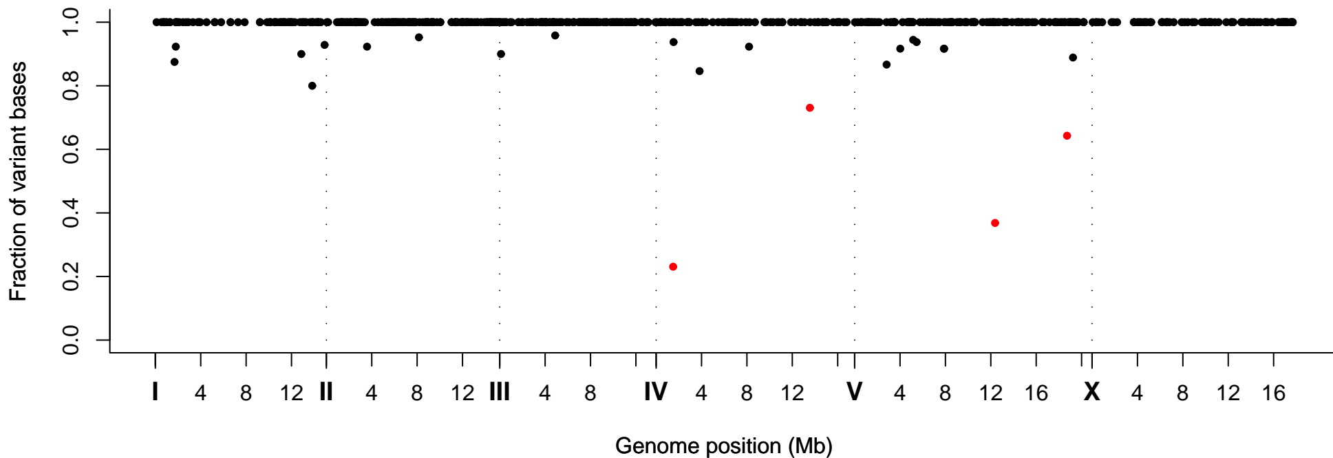
Fraction of Variant Bases at Position, Strain VC40607
