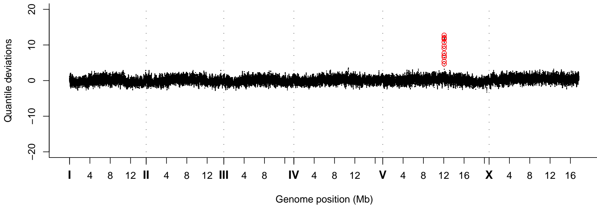
Quantile Deviations, Strain VC40626
