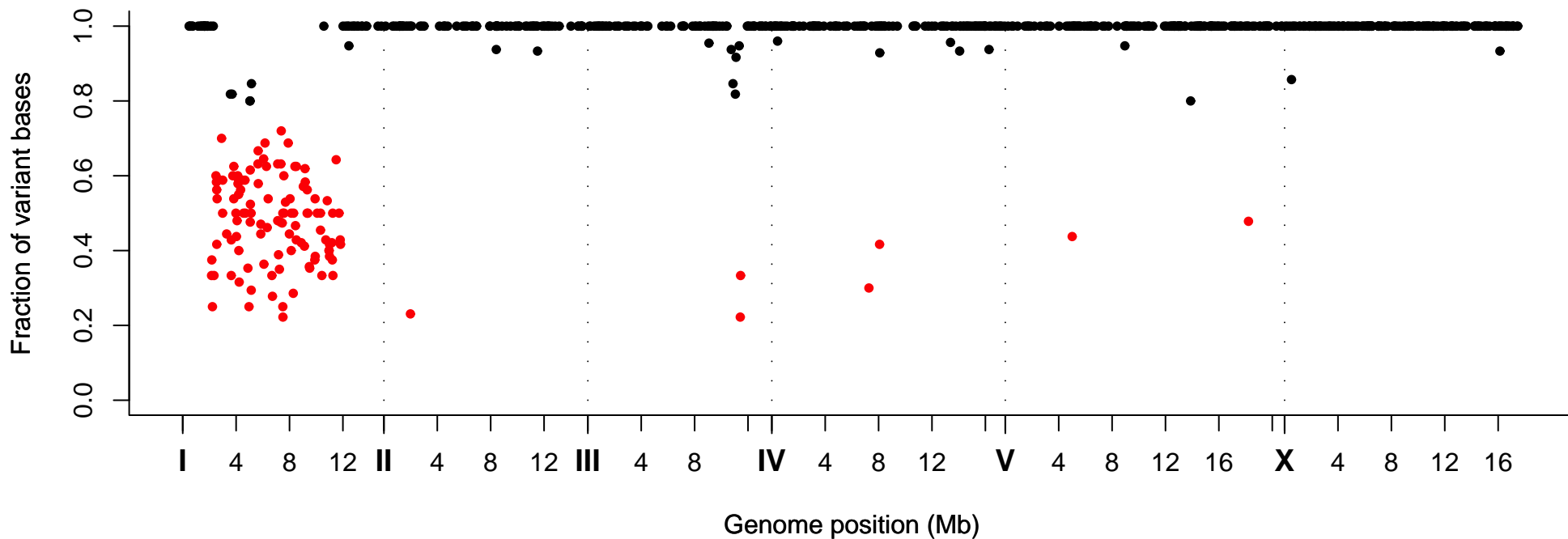
Fraction of Variant Bases at Position, Strain VC40626
