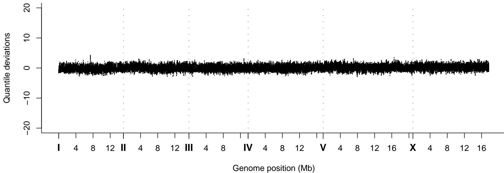
Quantile Deviations, Strain VC40638
