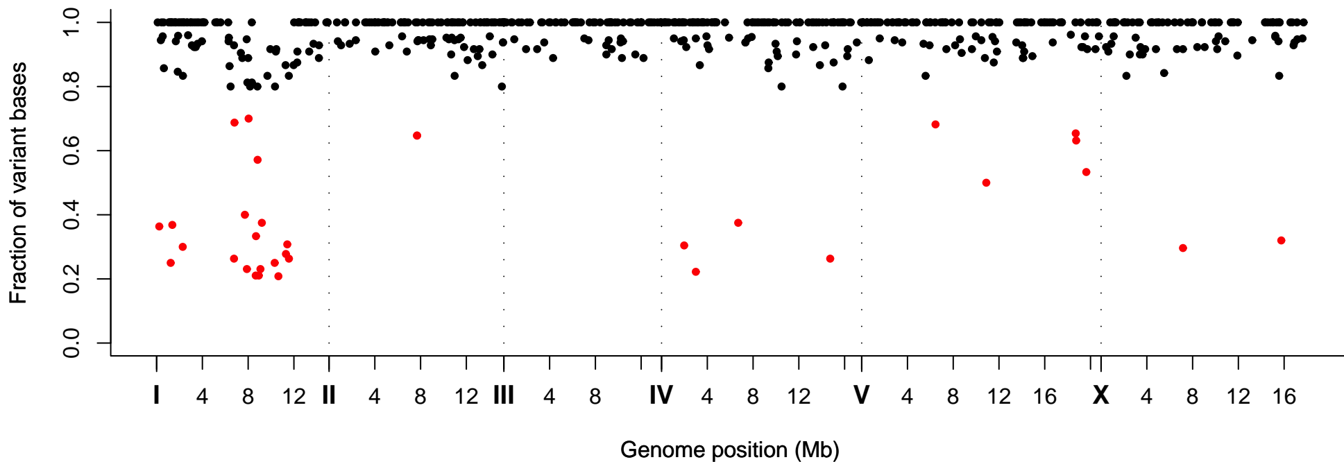
Fraction of Variant Bases at Position, Strain VC40638
