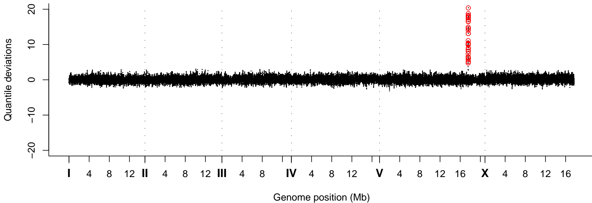
Quantile Deviations, Strain VC40643
