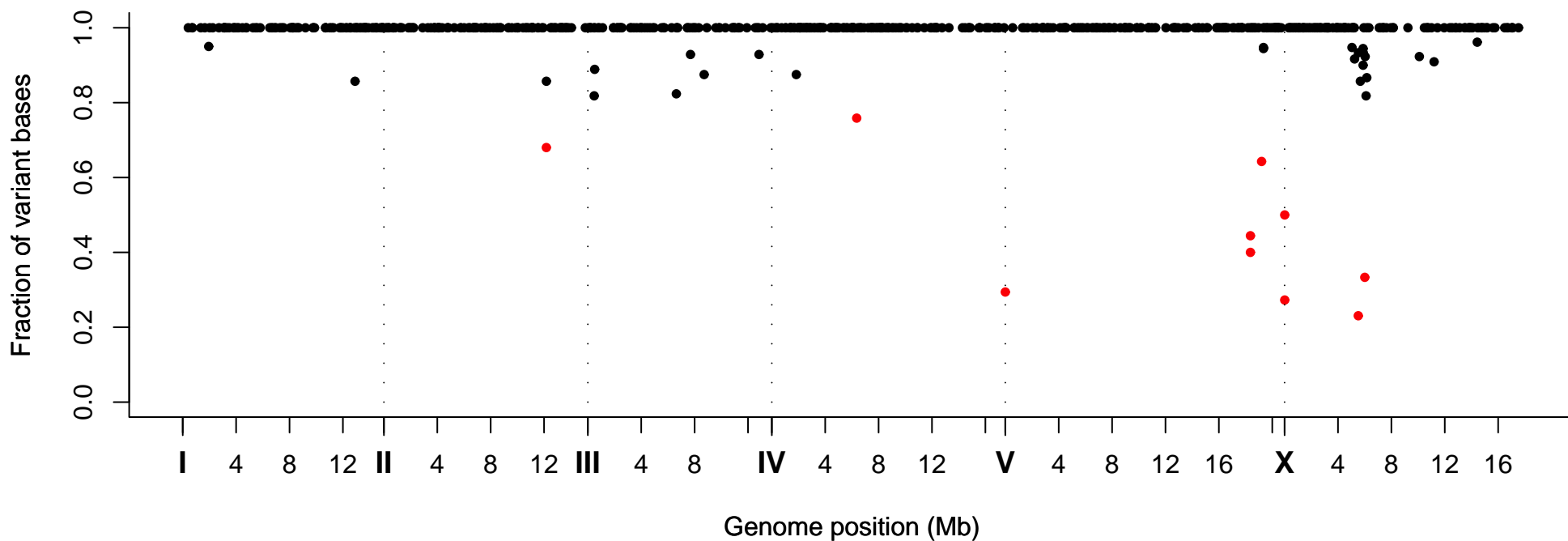
Fraction of Variant Bases at Position, Strain VC40643
