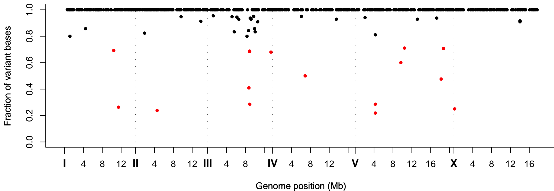
Fraction of Variant Bases at Position, Strain VC40649
