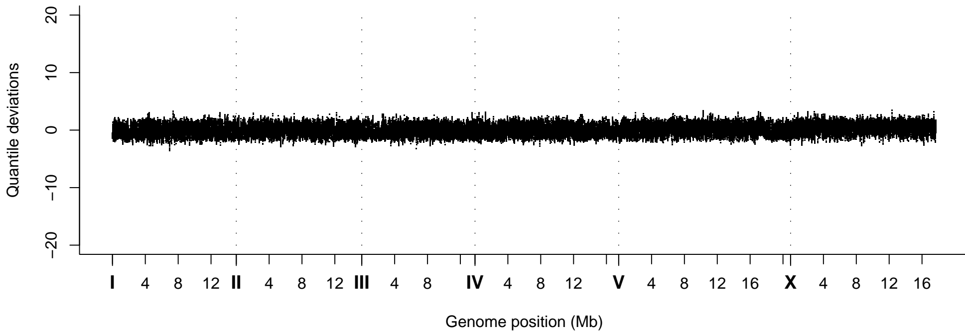
Quantile Deviations, Strain VC40649
