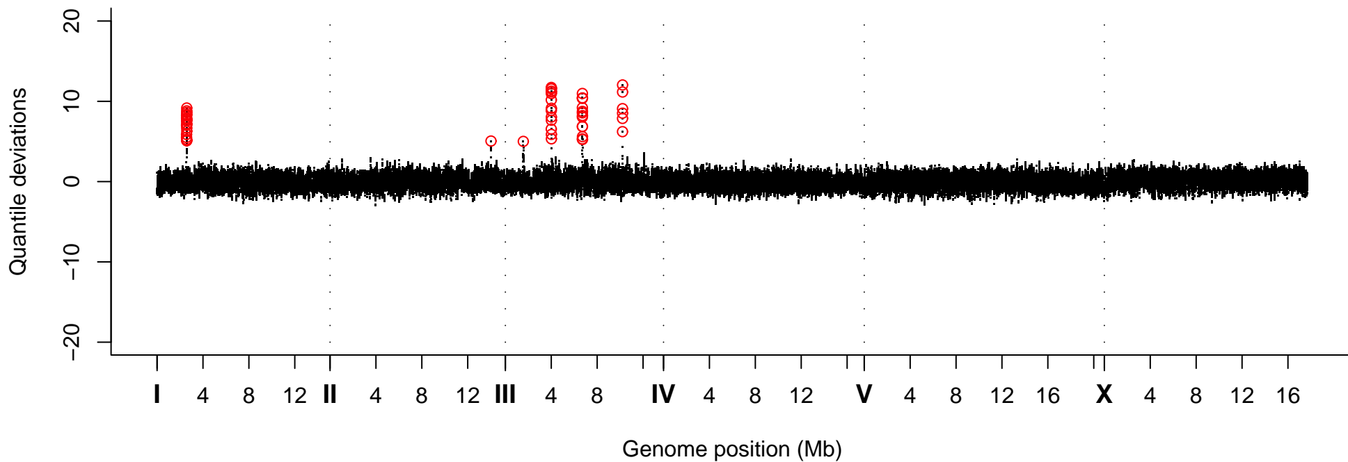
Quantile Deviations, Strain VC40658
