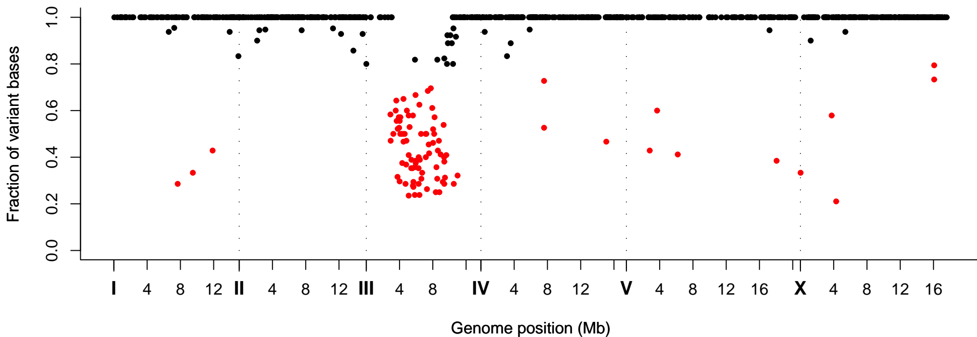
Fraction of Variant Bases at Position, Strain VC40658
