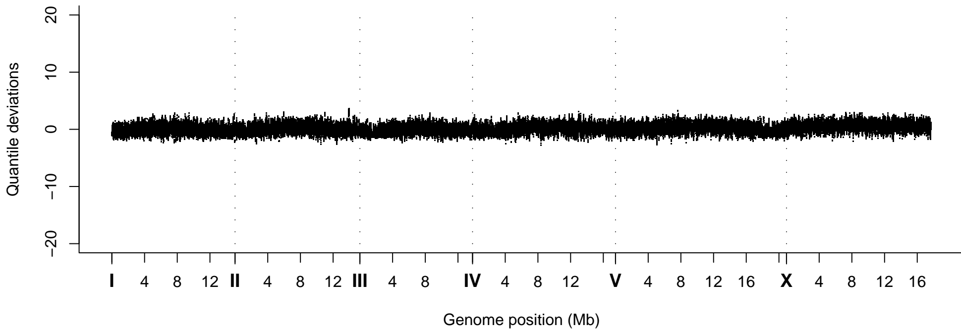
Quantile Deviations, Strain VC40661
