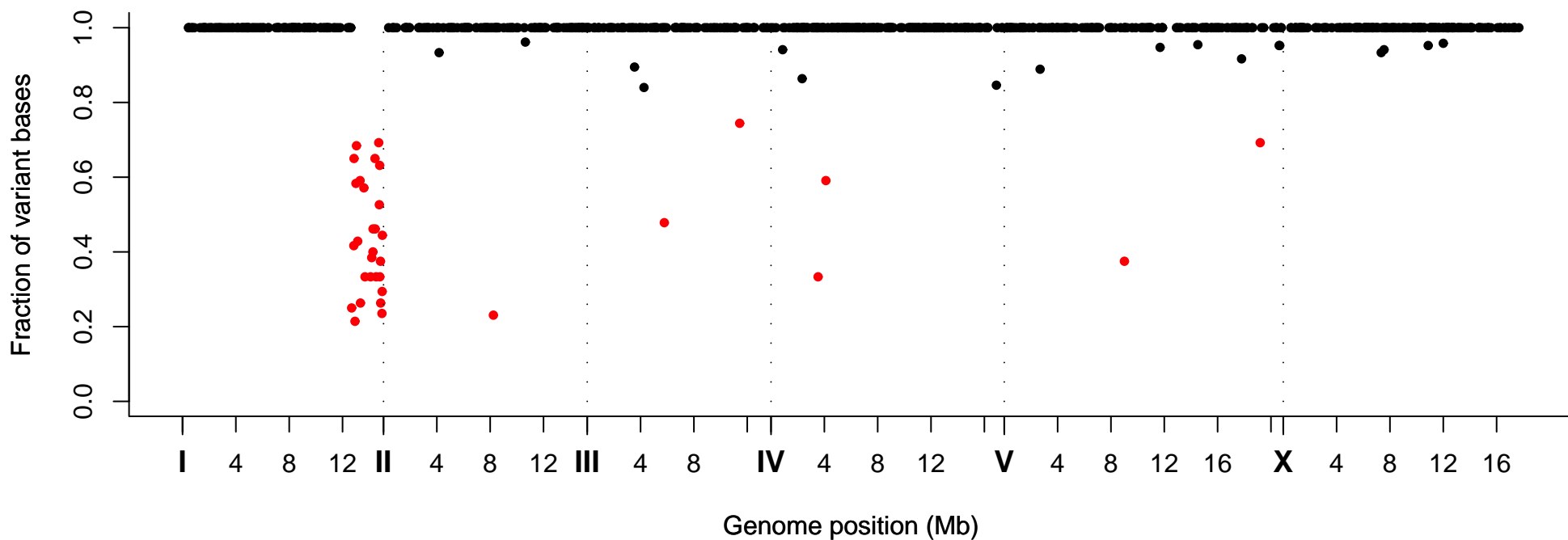
Fraction of Variant Bases at Position, Strain VC40661
