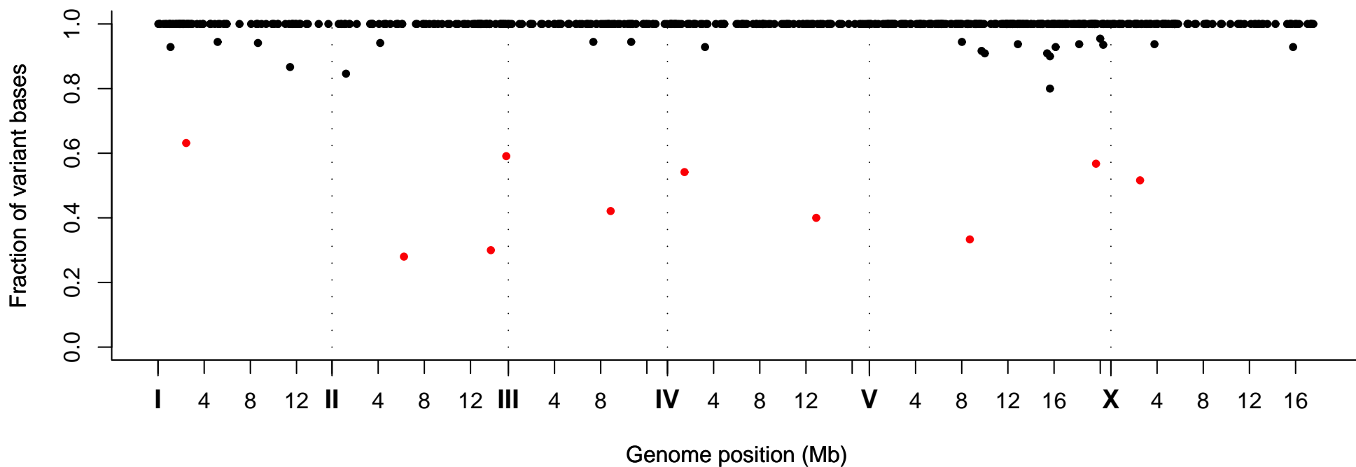
Fraction of Variant Bases at Position, Strain VC40665
